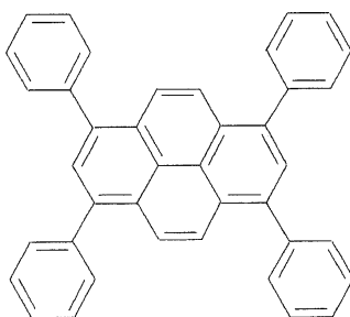
1, 3, 6, 8-테트라페닐페렌
