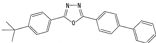
2-(4-tert-부틸페닐)-5-(4-비페닐릴)- 1, 3, 4-옥사졸
