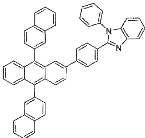
Compound 6
