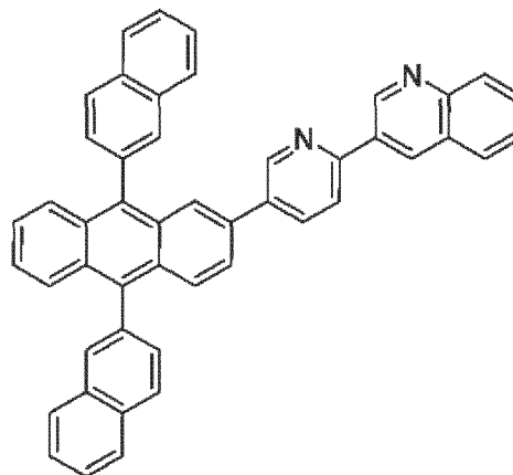
Compound 7.
