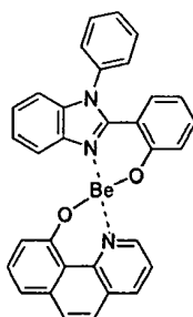
Compound 15
