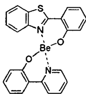
Compound 7
