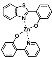
Compound 8
