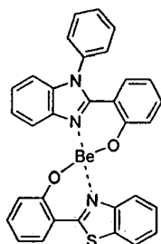
Compound 17
