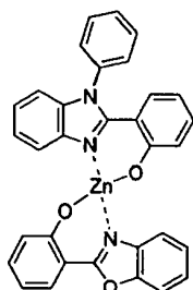
Compound 12
