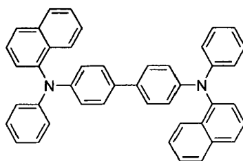
NPB
