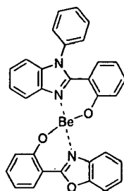
Compound 11
