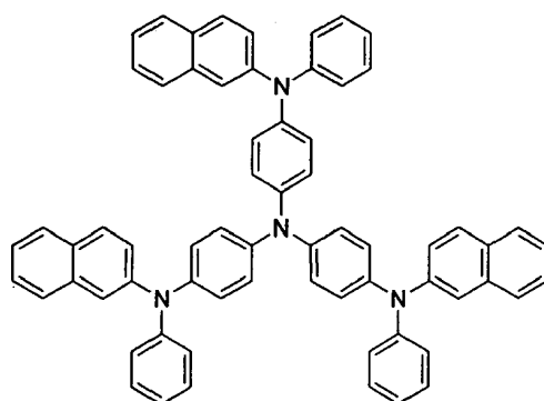
2-TNATA
