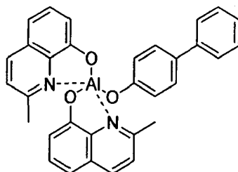
BAIq
