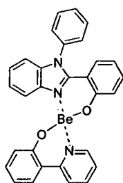
Compound 13
