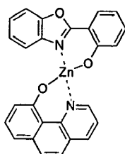
Compound 4
