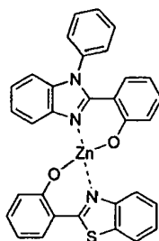
Compound 18
