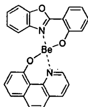
Compound 3
