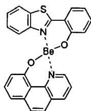
Compound 9
