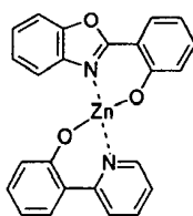
Compound 2
