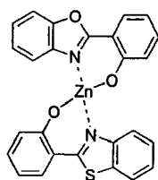
Compound 6
