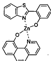
Compound 10
