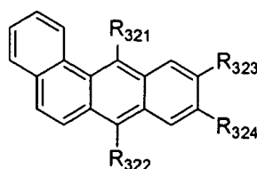
Chemical Formula 7
