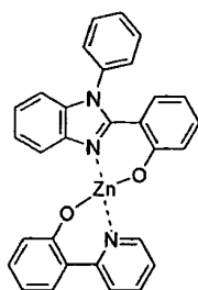
Compound 14
