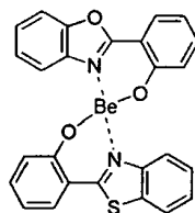
Compound 5
