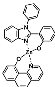
Compound 16
