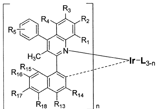
Chemical Formula 5
