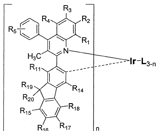
Chemical Formula 7
