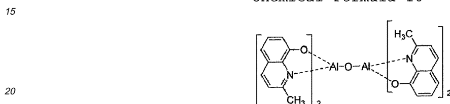
Chemical Formula 10
