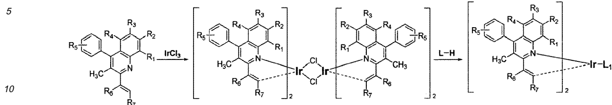
Reaction Scheme 2
