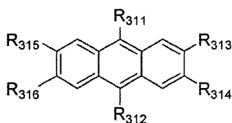
Chemical Formula 18
