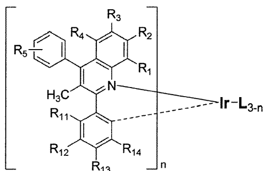
Chemical Formula 3
