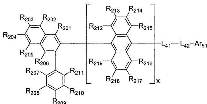
40 Chemical Formula 21
