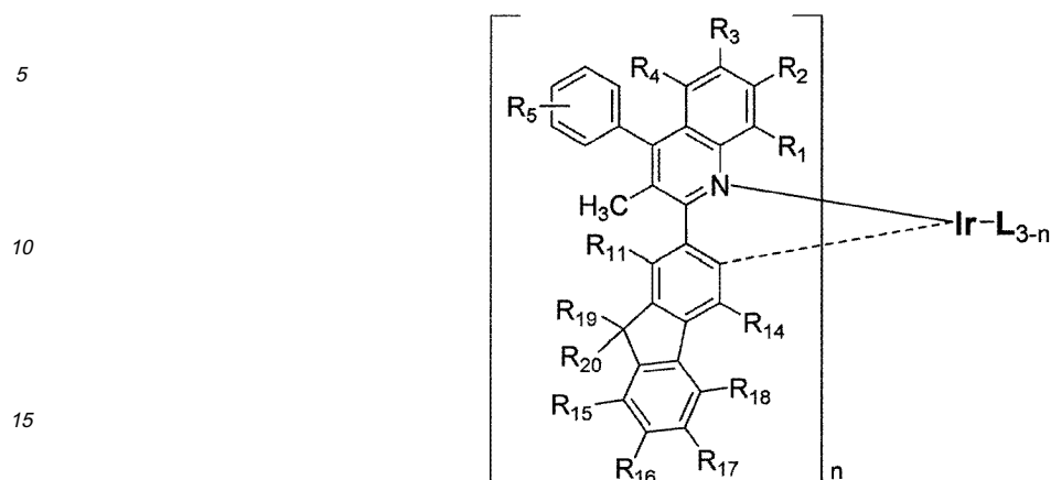
Chemical Formula 6
