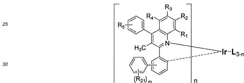
Chemical Formula 7
