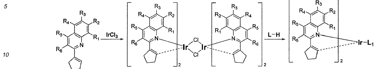
Reaction Scheme 2
