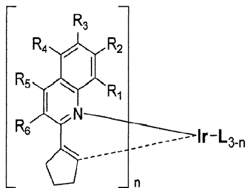
Chemical Formula 1
