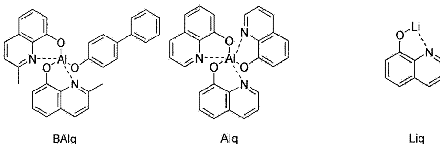
BAIq
