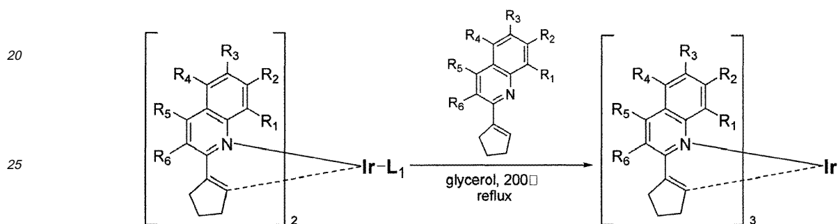
Reaction Scheme 3
