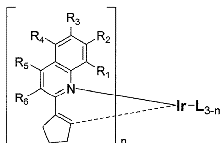
Chemical Formula 1
