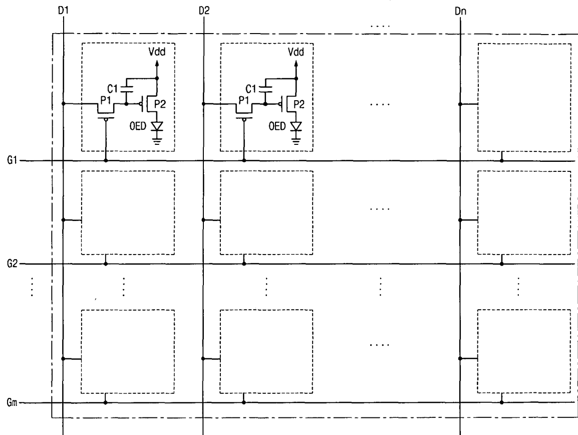
FIG. 1 RELATED ART
