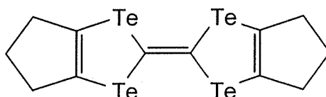
HMTTeF
