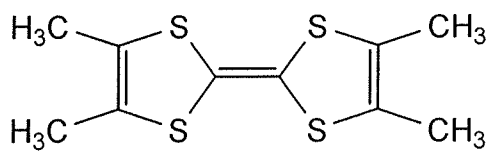
TMTTF
