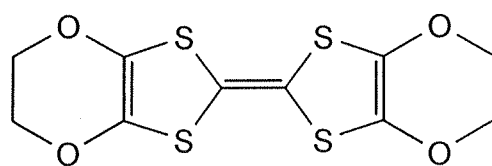
BEDO-TTF
