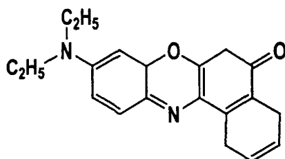
nile red
