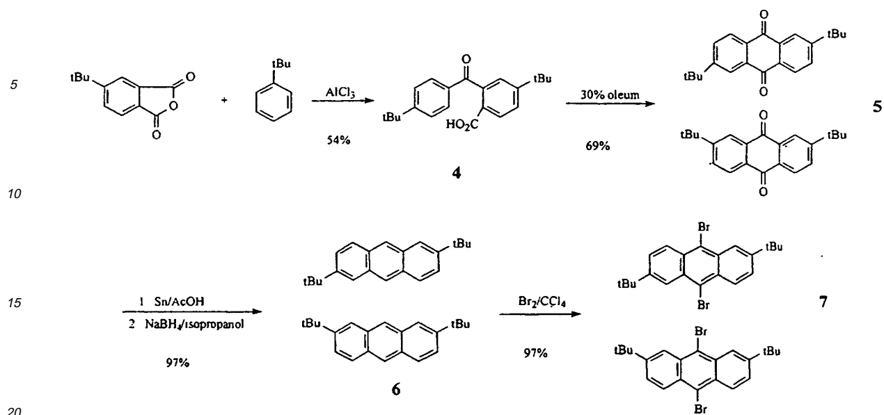
Scheme 2
