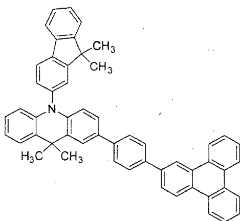
[Chemical Formula 74]
