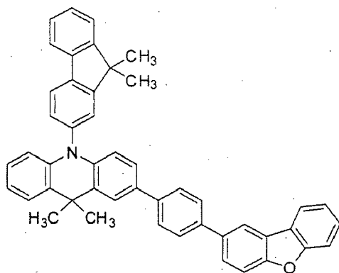
[Chemical Formula 81]
