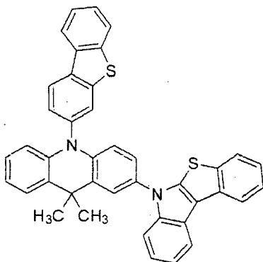
[Chemical Formula 5]
