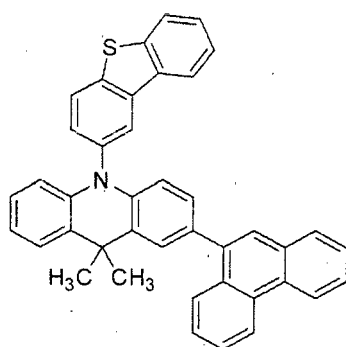
[Chemical Formula 43]
