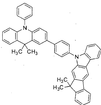
[Chemical Formula 38]
