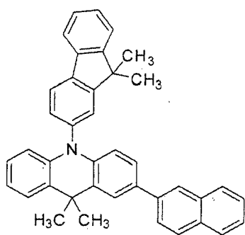
[Chemical Formula 72]
