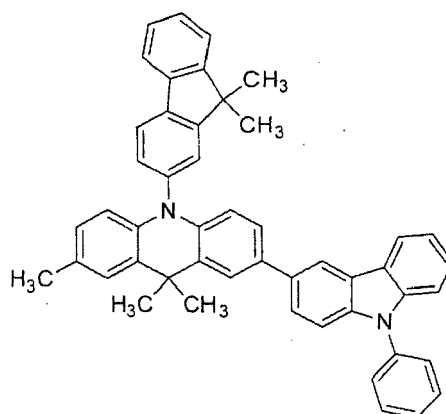
(Compound 69)
