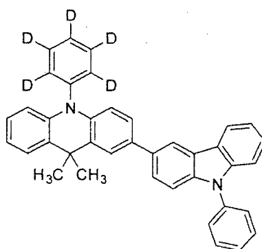
(Compound 32)
