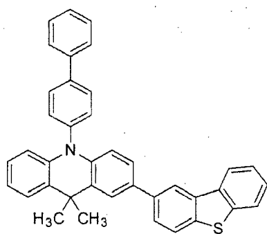
[Chemical Formula 11]
