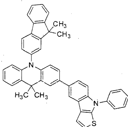
[Chemical Formula 40]
