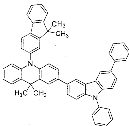
[Chemical Formula 16]
