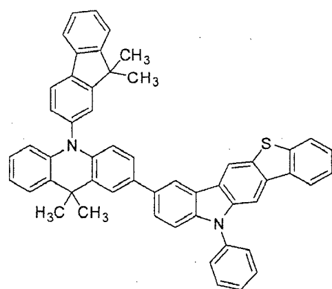
[Chemical Formula 28]
