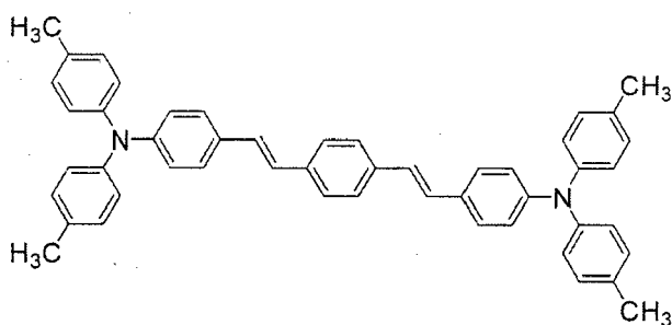
[Chemical Formula 87]
