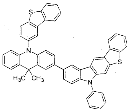
[Chemical Formula 27]
