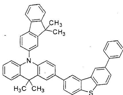
[Chemical Formula 17]
