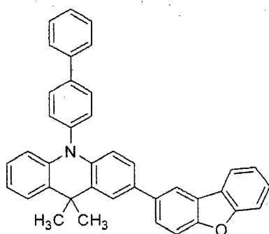
[Chemical Formula 12]
