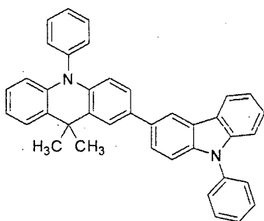
[Chemical Formula 8]
