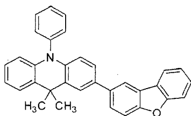
[Chemical Formula 65]
