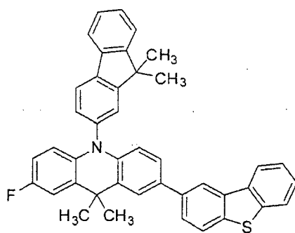
[Chemical Formula 63]
