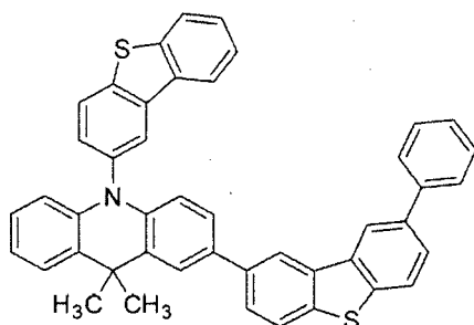
[Chemical Formula 66]
