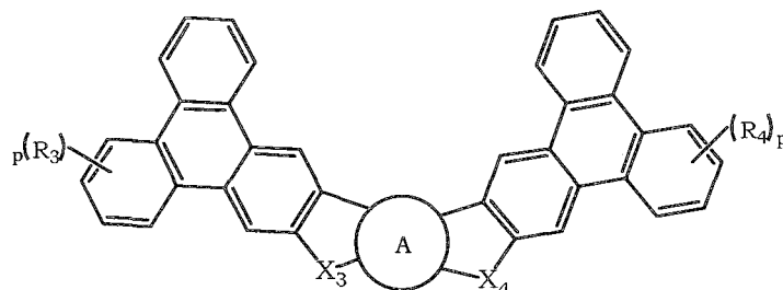
formula(II)
