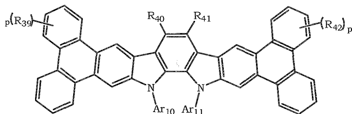
formula(II-3)
