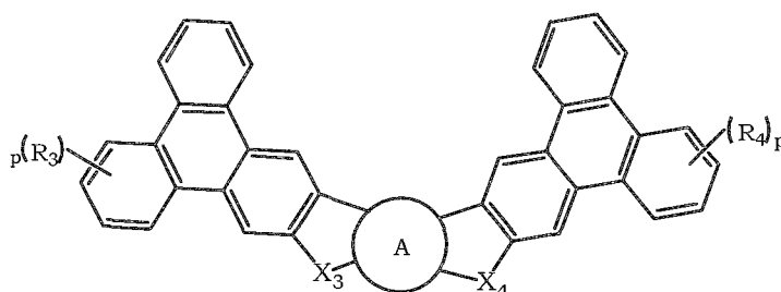
formula(II)
