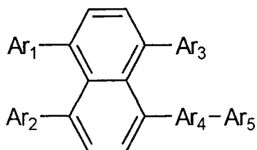
[Formula 1]
