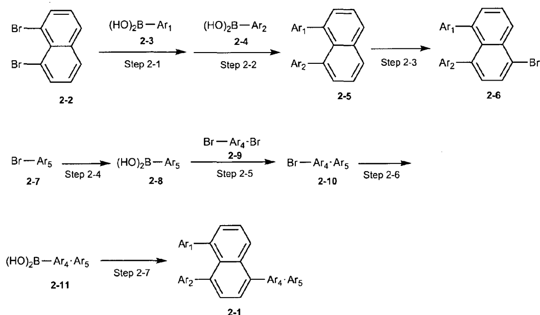
[Reaction scheme 2]
