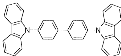
BCz
