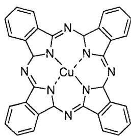
CuPc
