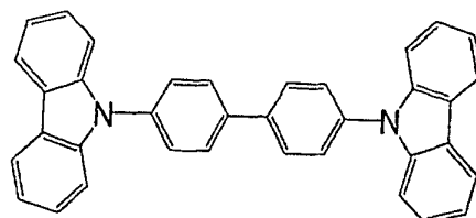
BCz
