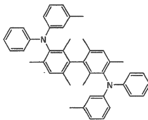
C-17
