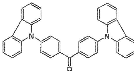
Comparative compound 8
