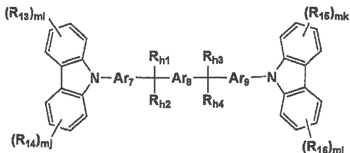
Formula H3
