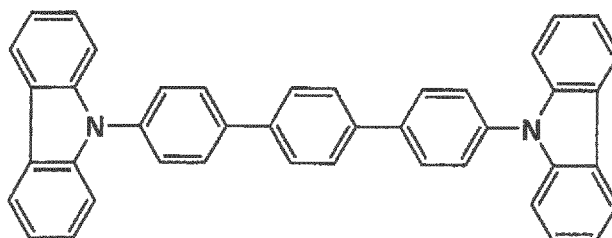
Comparative compound 4
