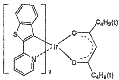
Ir-8
