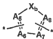
Formula (o)
