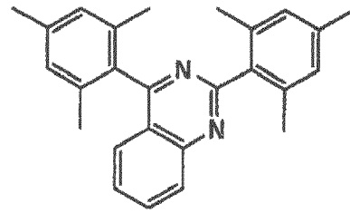
C1-2
