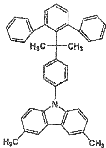
11-3
