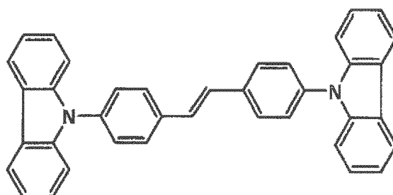
Comparative compound 7
