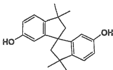
Bisphenol compound
