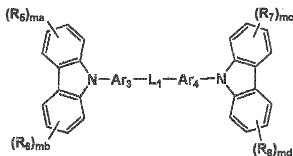
Formula H1
