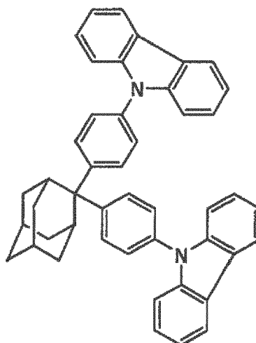
Comparative compound 8
