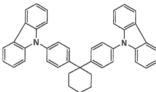
Comparative compound 2
