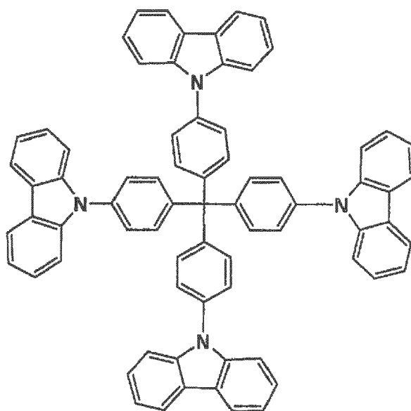
Comparative compound 12
