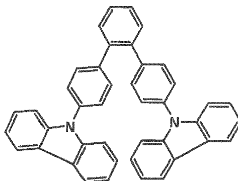
Comparative compound 4
