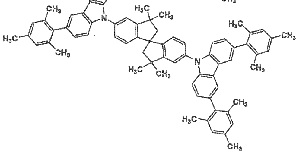
IA-4
