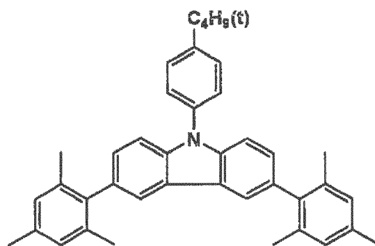
C-10
