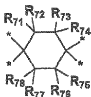
formula (h)
