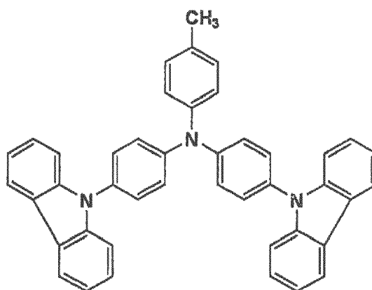
Comparative compound 2
