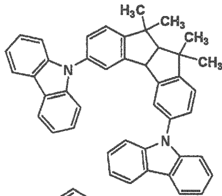
IA-12
