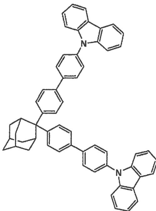
Comparative compound 1-1
