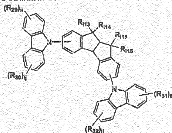
Formula I3
