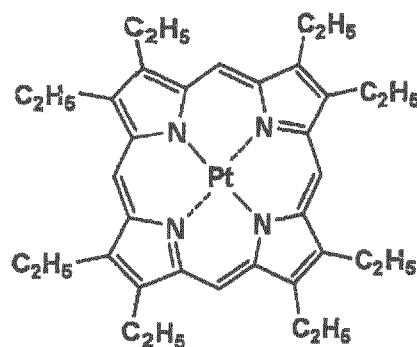
Pd-3
