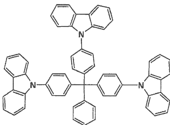
Comparative compound 12
