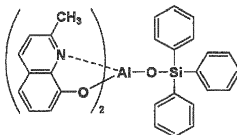
Compound A1
