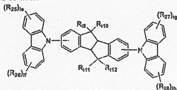
Formula I2
