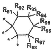
formula (j)
