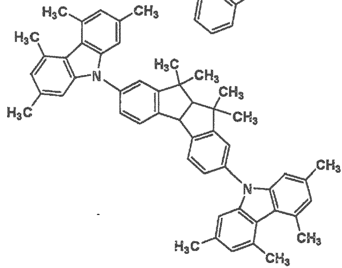
IA-14
