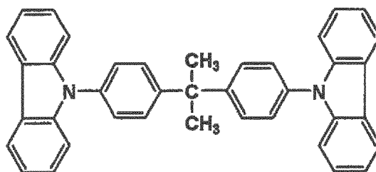
Comparative compound 10
