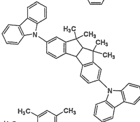
IA-13
