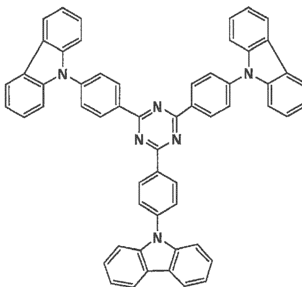
Comparative compound 10
