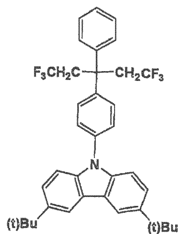
11-4
