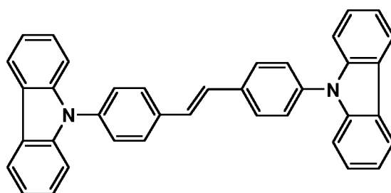
Comparative compound 6
