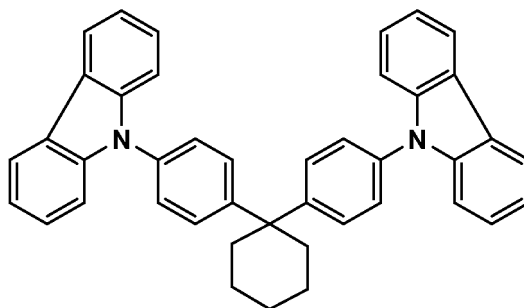
Comparative compound 2
