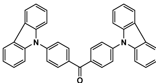
Comparative compound 8
