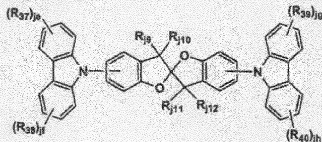
Formula J2
