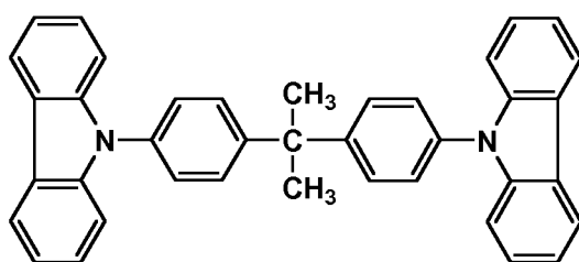
Comparative compound 9
