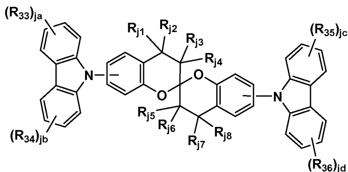
Formula J1
