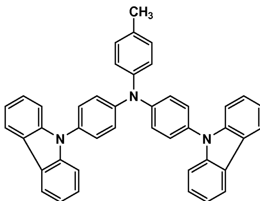
Comparative compound 1
