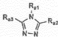
Formula 5
