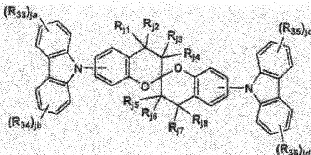
Formula J1
