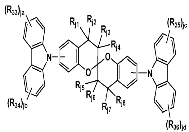
Formula J1
