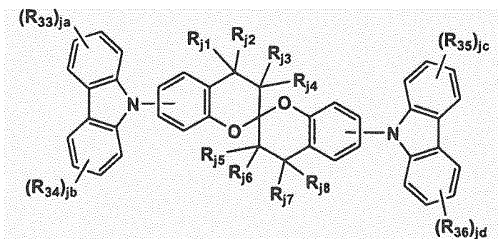
Formula J1
