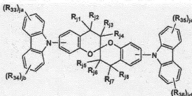
Formula J1
