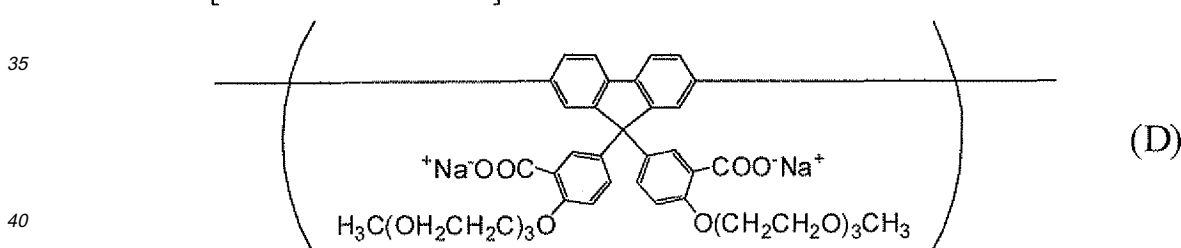
[Chemical formula 70]
