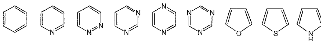
[Chemical formula 45]
