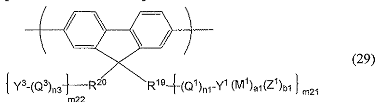
[Chemical formula 46]
