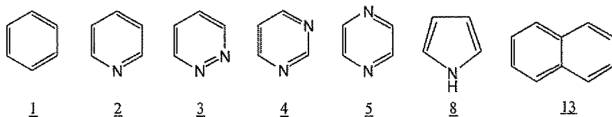
[Chemical formula 38]
