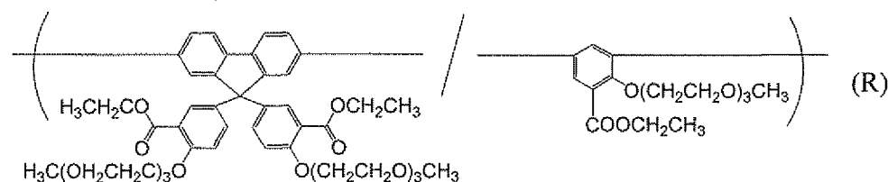
45 [Chemical formula 85]
