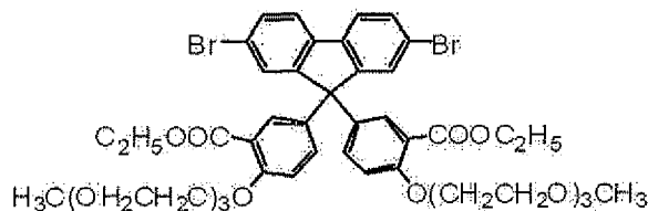
Compound A
