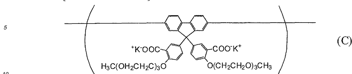
[Chemical formula 69]
