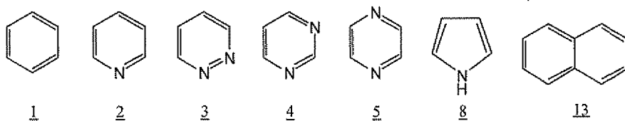
[Chemical formula 36]
