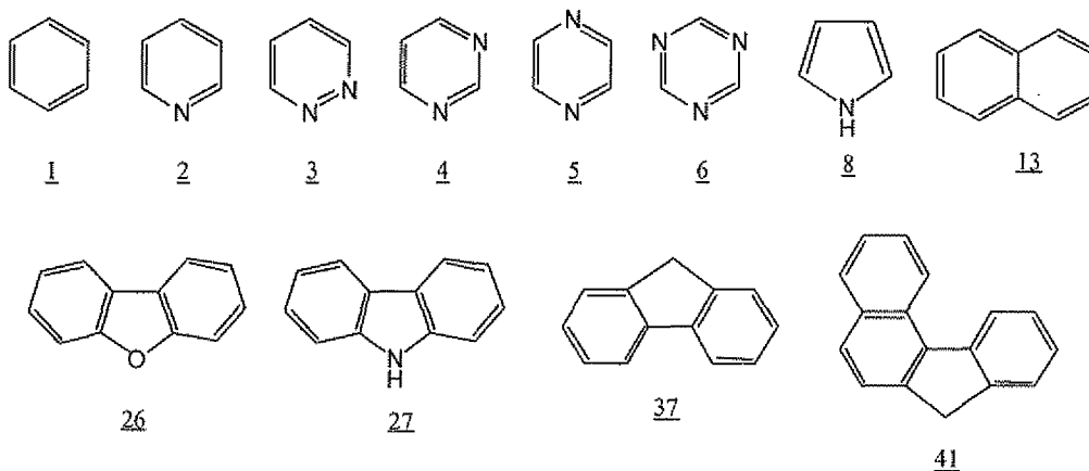
[Chemical formula 8]
