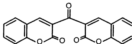
Chemical Formula 1
