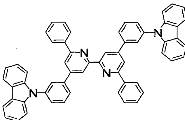
[ Chemical Formula 100]
