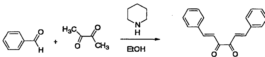
Target Compound 11
