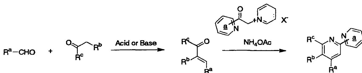
[ Chemical Formula 29 ]
