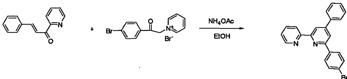
Target Compound 22
