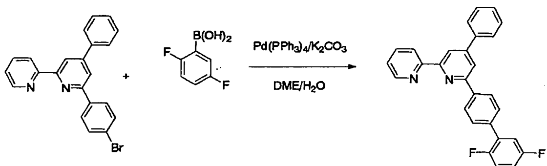
Target Compound 23
