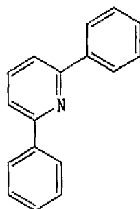
Chemical Formula 13
