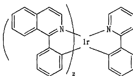
Chemical Formula 17
