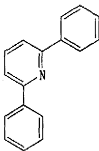
Chemical Formula 13
