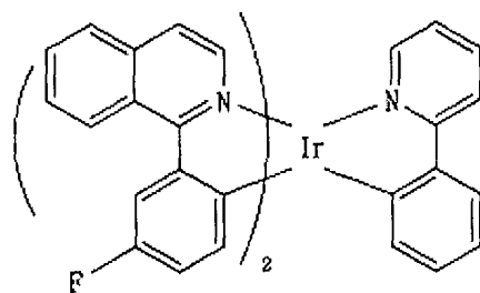
Chemical Formula 20
