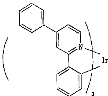
Chemical Formula 30
