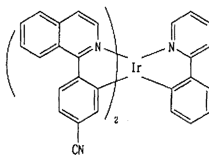
Chemical Formula 19
