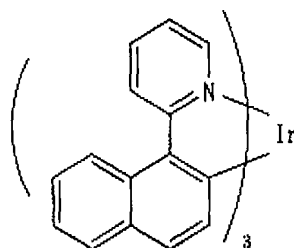
Chemical Formula 26
