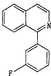
Chemical Formula 12
