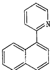
Chemical Formula 4
