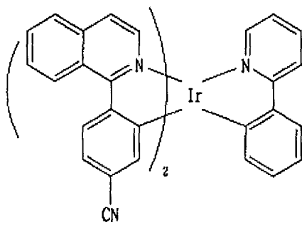
Chemical Formula 18
