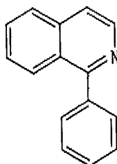
Chemical Formula 5
