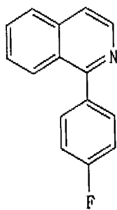
Chemical Formula 7
