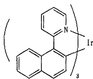
Chemical Formula 26
