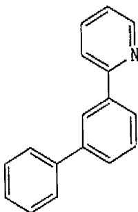
Chemical Formula 3
