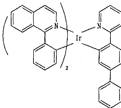
Chemical Formula 21
