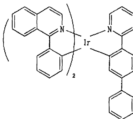
Chemical Formula 22
