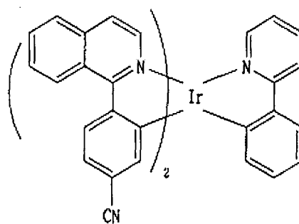
Chemical Formula 18
