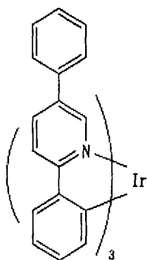
Chemical Formula 23
