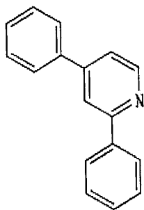
Chemical Formula 8
