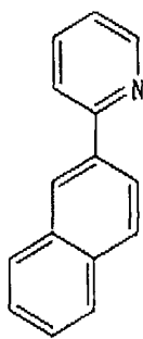
Chemical Formula 10
