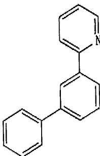
Chemical Formula 3
