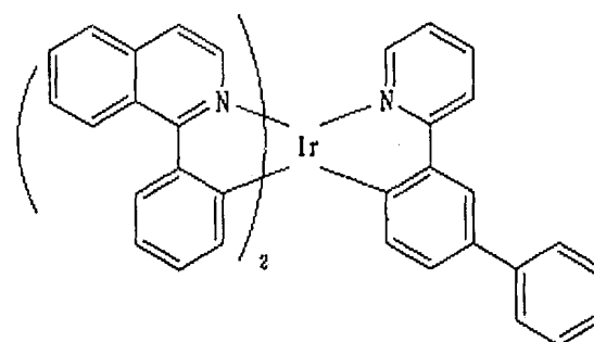
Chemical Formula 22
