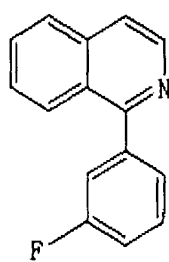
Chemical Formula 12
