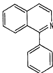
Chemical Formula 6
