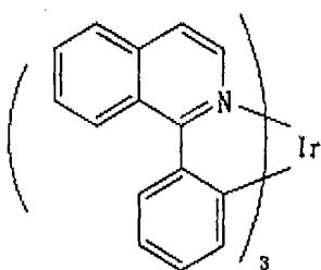
Chemical Formula 27
