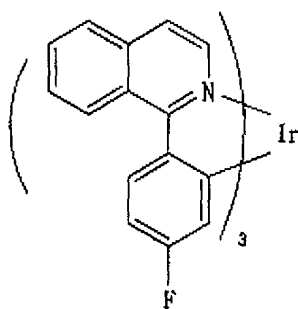
Chemical Formula 29
