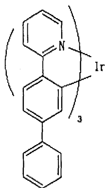
Chemical Formula 24
