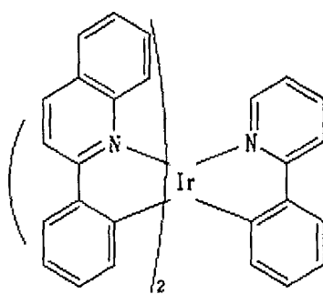
Chemical Formula 16
