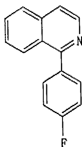
Chemical Formula 7
