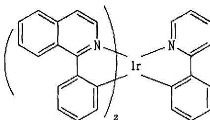
Chemical Formula 17
