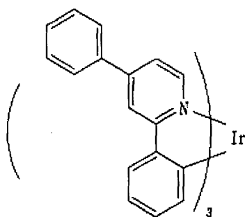
Chemical Formula 30
