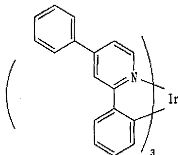
Chemical Formula 30
