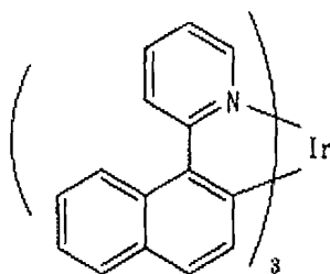
Chemical Formula 26
