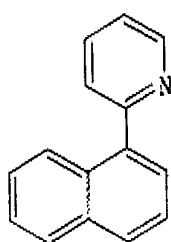
Chemical Formula 4
