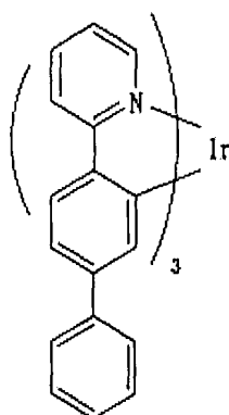
Chemical Formula 24
