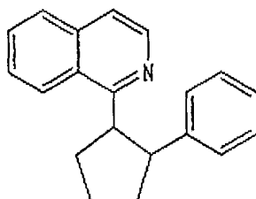
Chemical Formula 14
