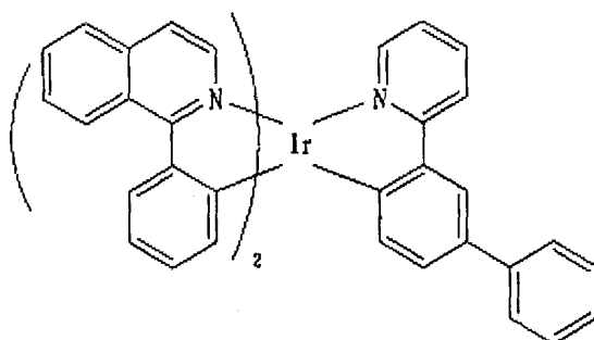
Chemical Formula 22
