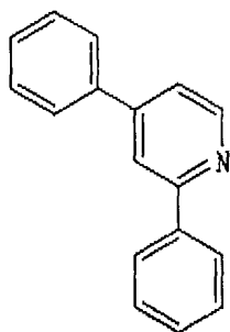
Chemical Formula 9
