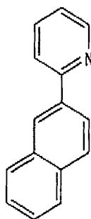
Chemical Formula 9
