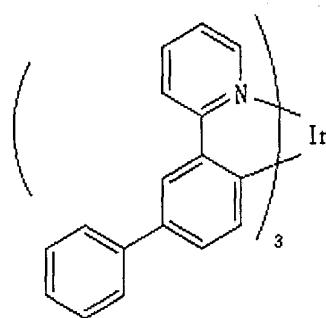
Chemical Formula 26
