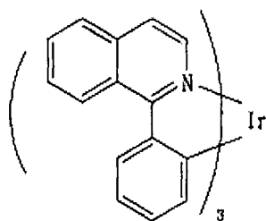
Chemical Formula 27
