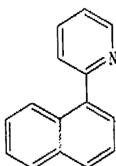
Chemical Formula 4
