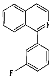
Chemical Formula 12
