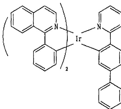
Chemical Formula 21
