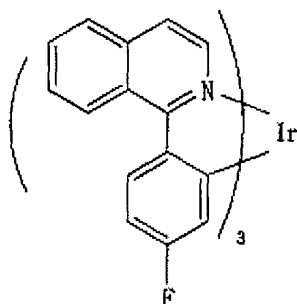
Chemical Formula 29
