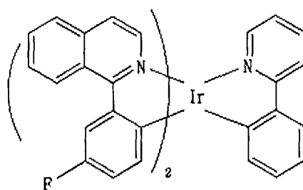
Chemical Formula 19
