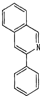
Chemical Formula 10
