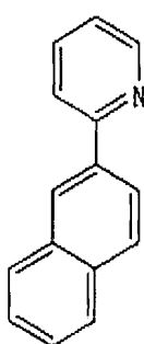
Chemical Formula 9
