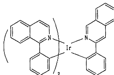
Chemical Formula 20
