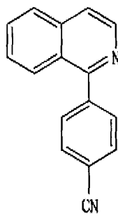
Chemical Formula 11
