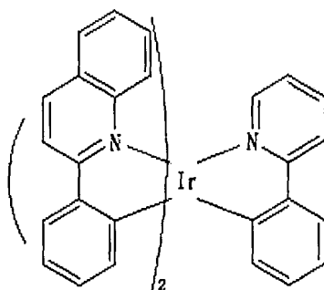
Chemical Formula 16
