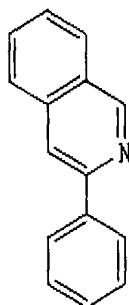
Chemical Formula 10
