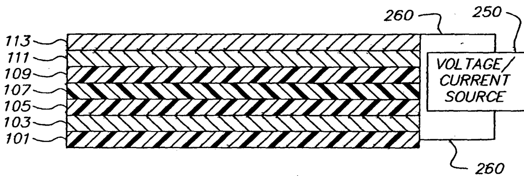
FIG. 3 (PRIOR ART)
