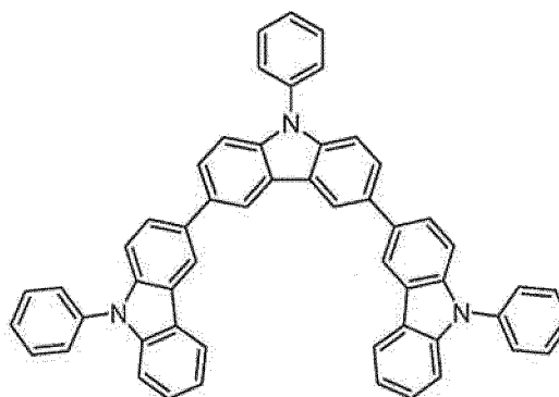
TrisPCz
