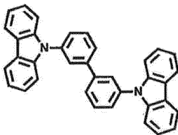
mCBP
