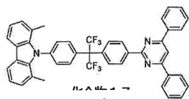
Compound 17
