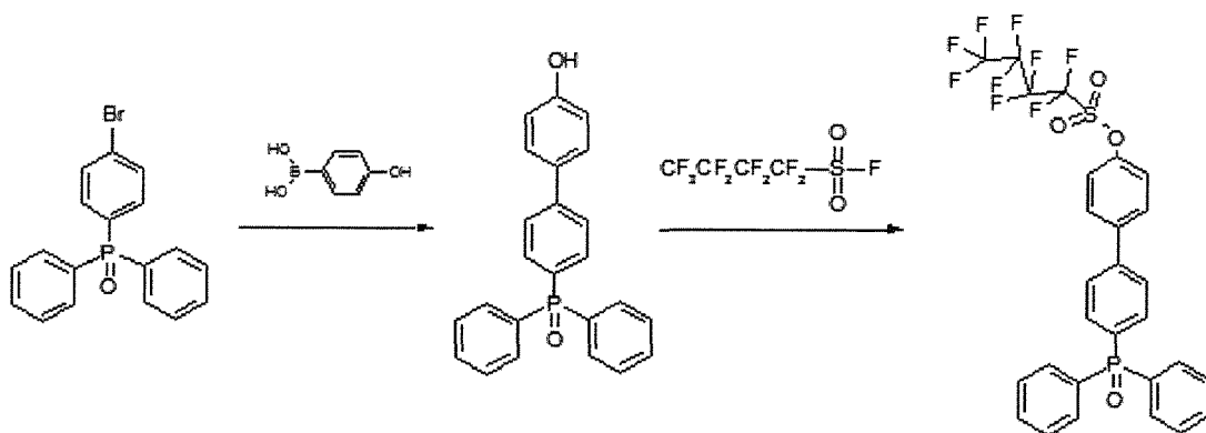
Structural Formula 1-7E
