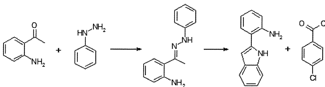
Structural Formula 1-2A Structural Formula 1-2B
