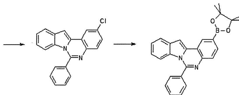
Structural Formula 1-7C
