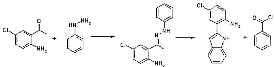
Structural Formula 1-7A Structural Formula 1-7B
