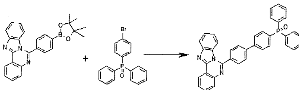
Structural Formula 1-2
