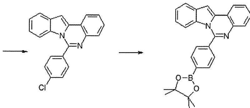
Structural Formula 1-2C
