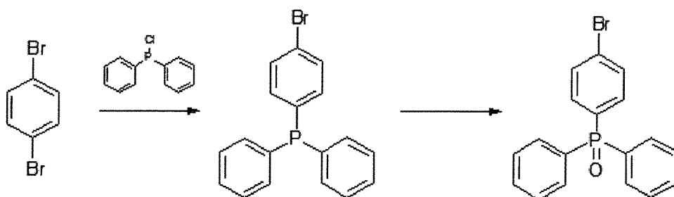
Structural Formula 1-2E
