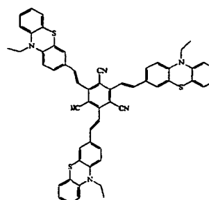
Compound 18
