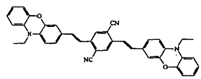
Compound 4
