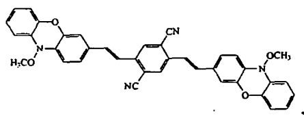
Compound 5
