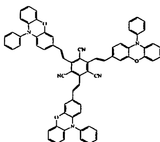
Compound 17
