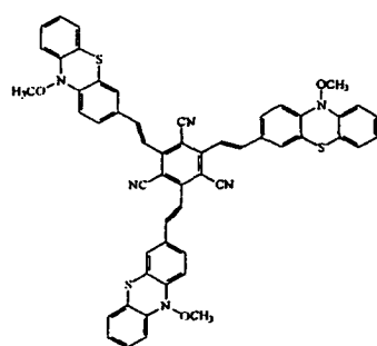
Compound 19
