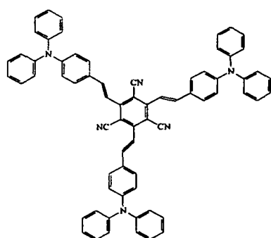
Compound 21
