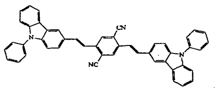
Compound 3
