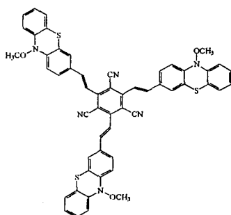
Compound 19
