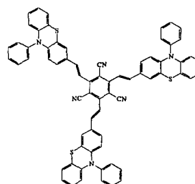
Compound 20
