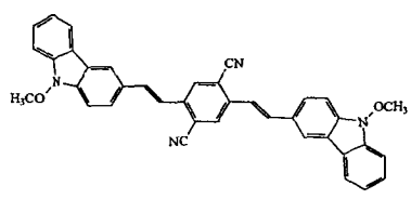
Compound 2
