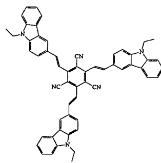
Compound 12
