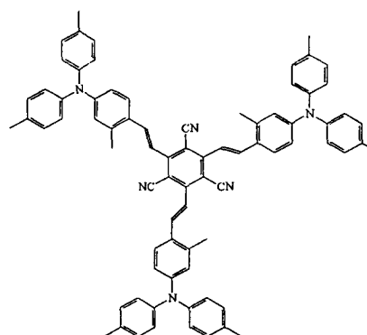
Compound 22
