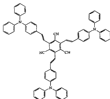
Compound 21
