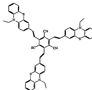
Compound 18
