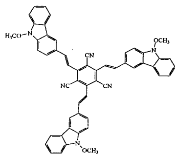
Compound 13
