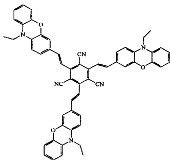
Compound 15
