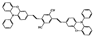
Compound 6
