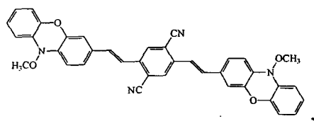
Compound 5
