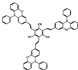
Compound 17
