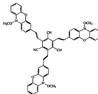
Compound 16
