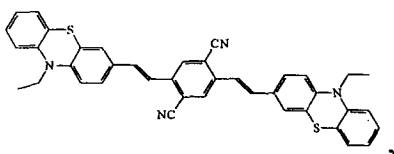
Compound 7
