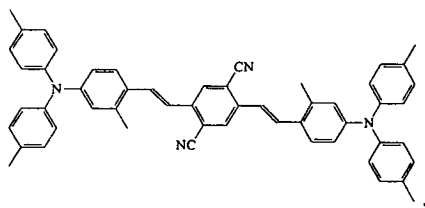
Compound 11
