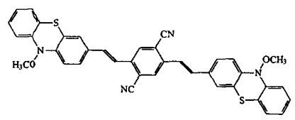
Compound 8
