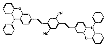
Compound 6
