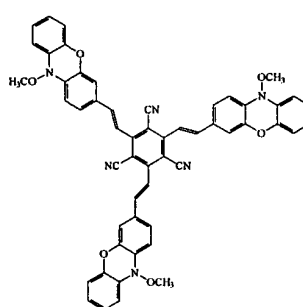
Compound 16
