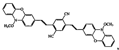
Compound 5
