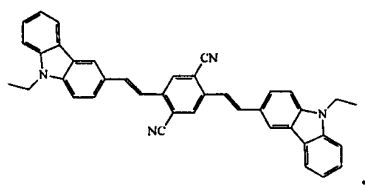
Compound 1
