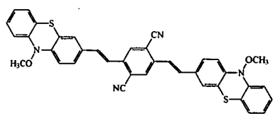
Compound 8
