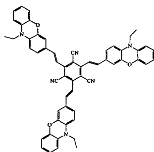
Compound 15
