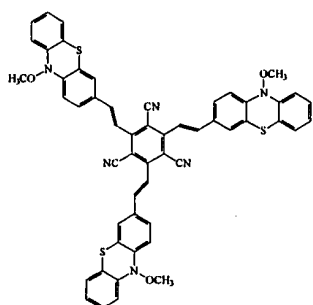
Compound 19
