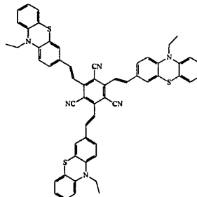
Compound 18
