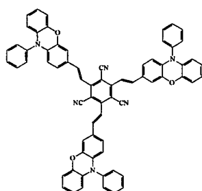
Compound 17
