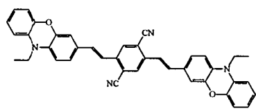
Compound 4
