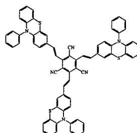
Compound 20
