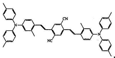
Compound 11
