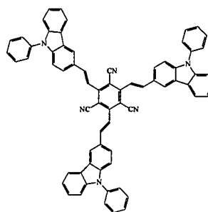
Compound 14
