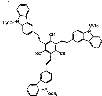
Compound 13
