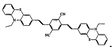
Compound 7
