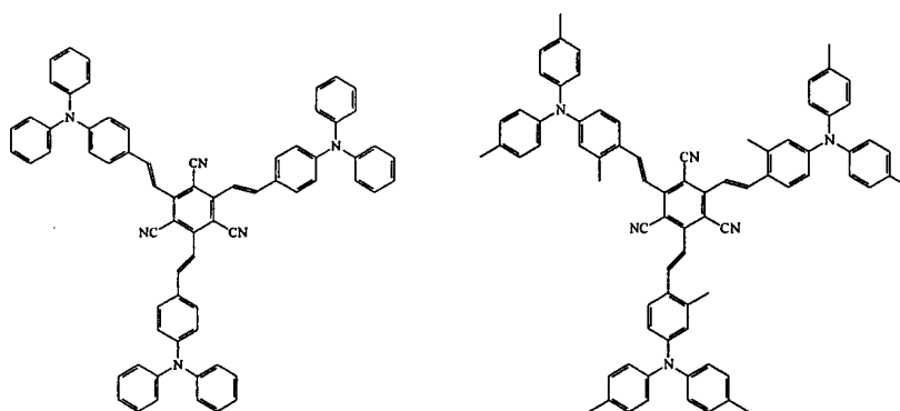
Compound 21
