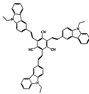
Compound 12
