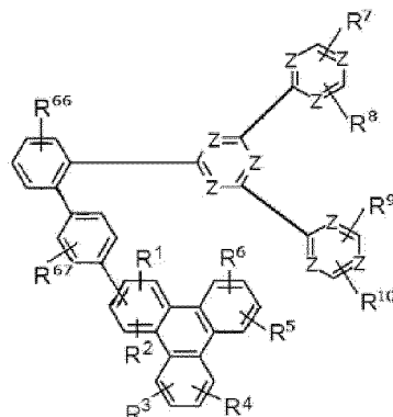
[Chemical Formula 1n]
