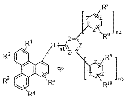
[Chemical Formula 1-II]
