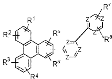
[Chemical Formula 1b]
