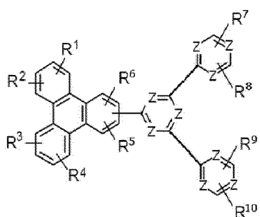
[Chemical Formula 1b]
