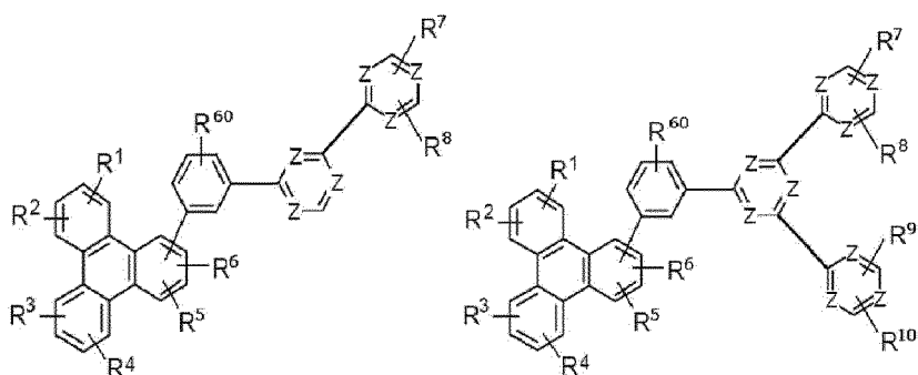
[Chemical Formula 1c]
