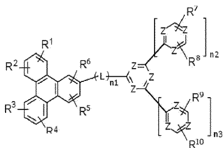
[Chemical Formula 1-II]
