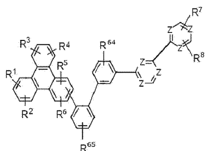
[Chemical Formula 1i]
