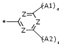
[Chemical Formula A]
