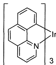
\text{Ir}(\text{bzq})_3
