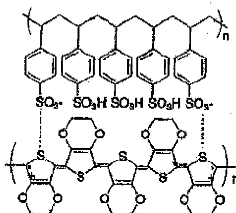
[Chemical Formula 1]
