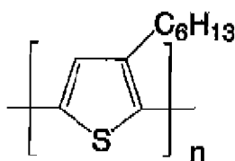
poly(3-hexylthiophene)
