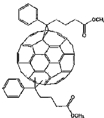
[Chemical Formula 3]
