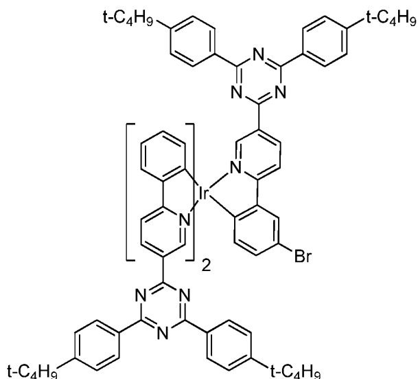
Monomer H
