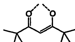
dipivaloylmetanate
