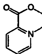
Picolinate
