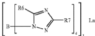
Chemical Formula 9
