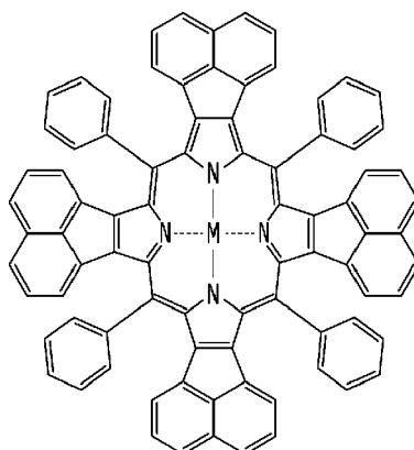
Chemical Formula 1-4
