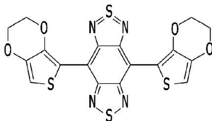
Chemical Formula 4
