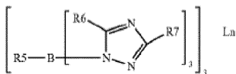
Chemical Formula 7
