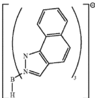
Chemical Formula 5-2-1
