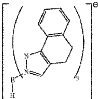
Chemical Formula 5-2-2
