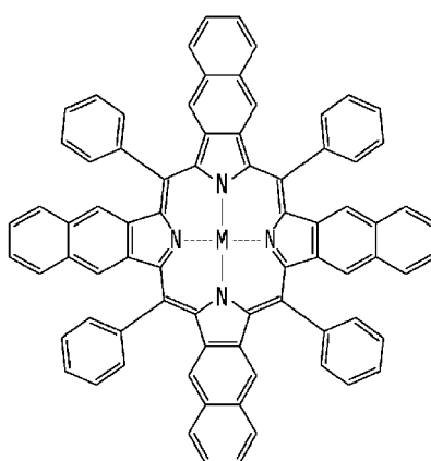
Chemical Formula 1-6
