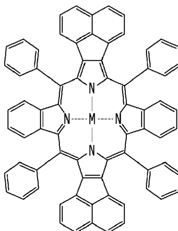
Chemical Formula 1-5
