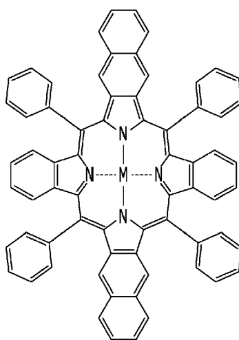
Chemical Formula 1-2
