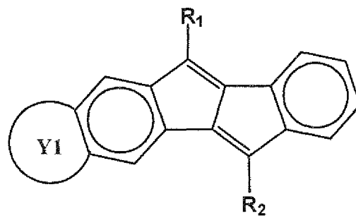
[Chemical Formula 5]
