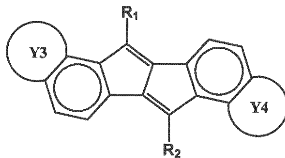
[Chemical Formula 7]
