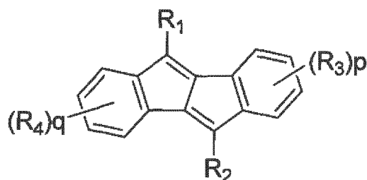
[Chemical Formula 9]
