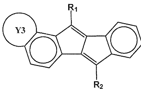
[Chemical Formula 7]
