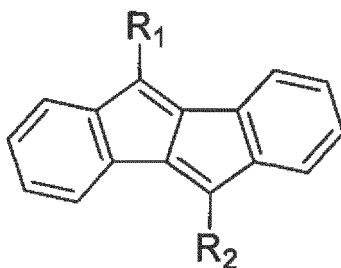
[Chemical Formula 3]
