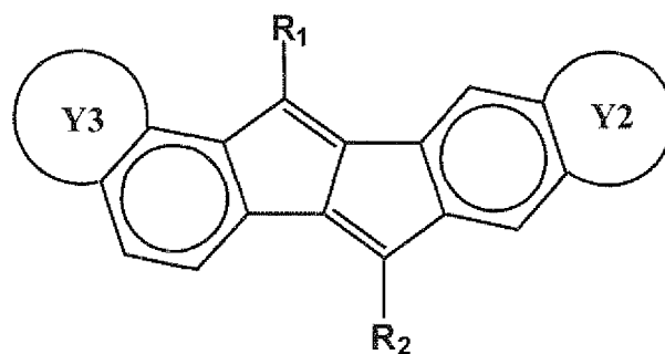
[Chemical Formula 8]
