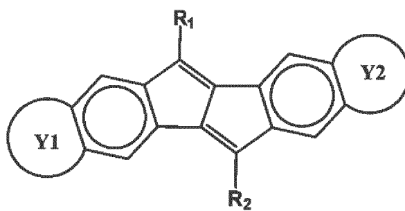
[Chemical Formula 6]
