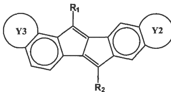
[Chemical Formula 9]
