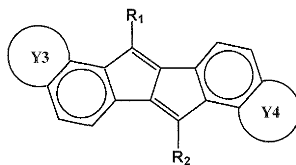
[Chemical Formula 8]
