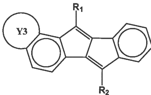
[Chemical Formula 7]
