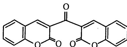
Chemical formula1
