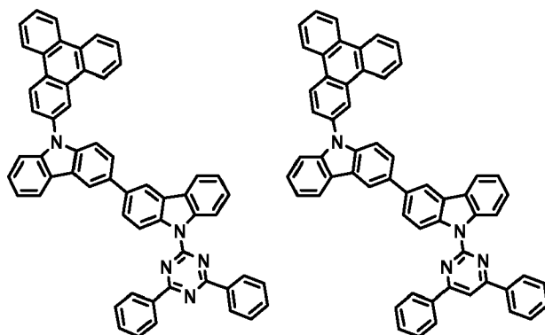
[Chemical Formula 47] [Chemical Formula 48]
