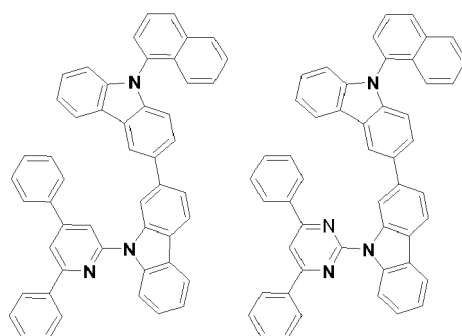
[Chemical Formula A-26]
