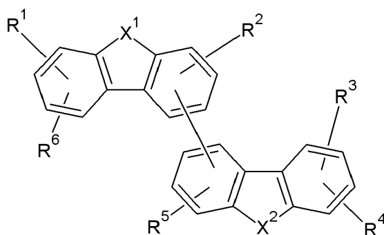
[Chemical Formula 1]
