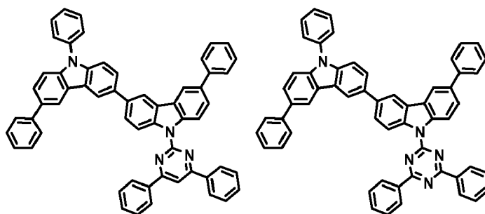
[Chemical Formula 15] [Chemical Formula 16]
