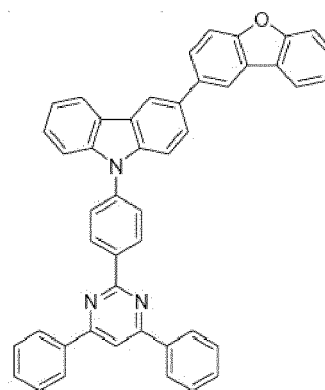
[Chemical Formula B-18] [Chemical Formula B-19] [Chemical Formula B-20]
