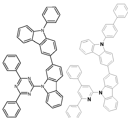
[Chemical Formula A-20] [Chemical Formula A-21]
