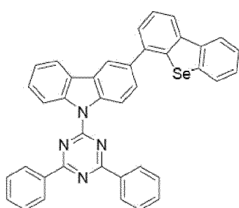
[Chemical Formula B-12] [Chemical Formula B-13] [Chemical Formula B-14]
