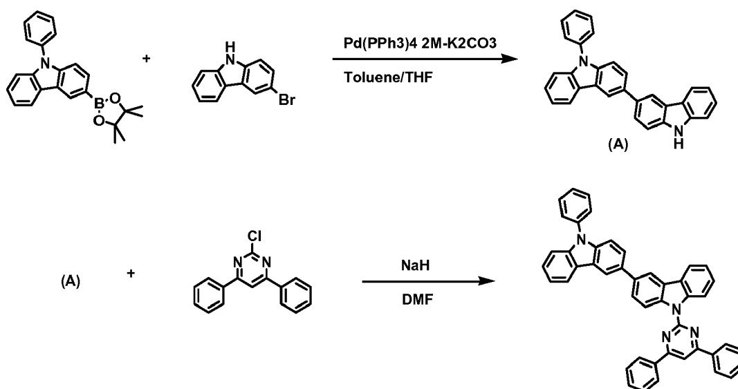
[Reaction Scheme 1]
