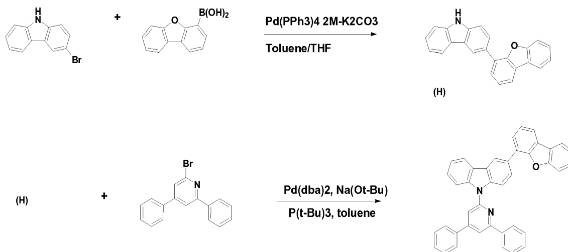
[Reaction Scheme 8]
