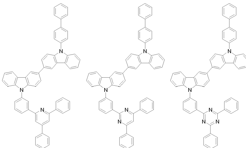
[Chemical Formula C-16] [Chemical Formula C-17] [Chemical Formula C-18]
