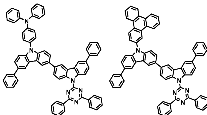
[Chemical Formula 41] [Chemical Formula 42]
