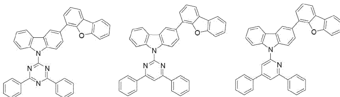
[Chemical Formula B-12] [Chemical Formula B-13] [Chemical Formula B-14]
