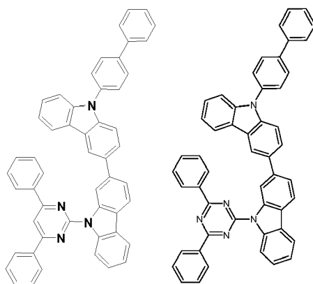
[Chemical Formula A-24] [Chemical Formula A-25]
