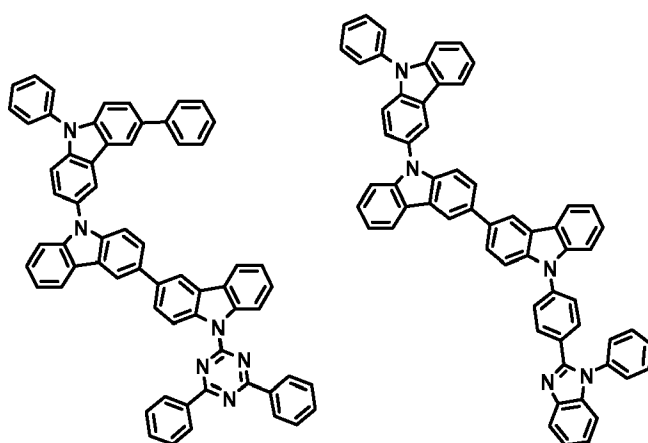
[Chemical Formula 29] [Chemical Formula 30]
