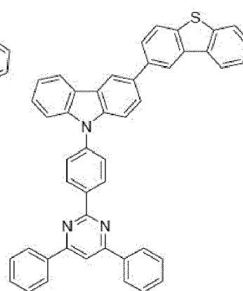
[Chemical Formula B-15] [Chemical Formula B-16] [Chemical Formula B-17]
