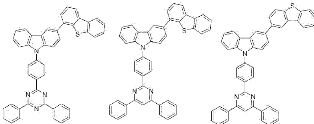
[Chemical Formula B-12] [Chemical Formula B-13] [Chemical Formula B-14]
