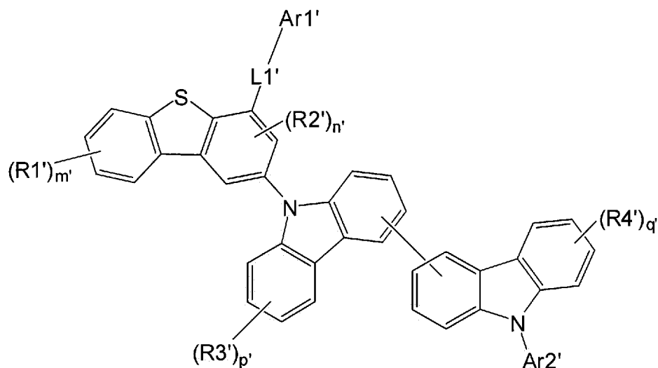
[Chemical Formula 2]
