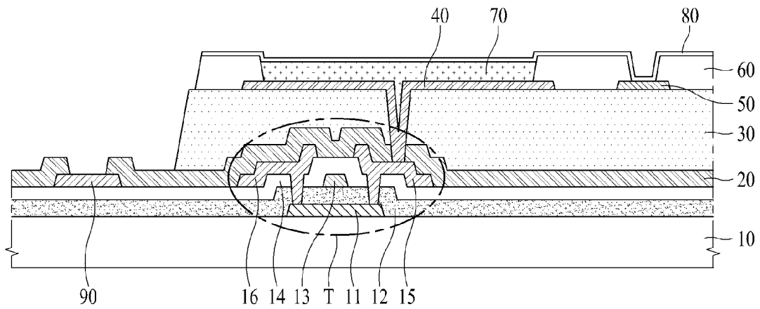
FIG. 1 (RELATED ART)
