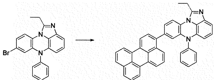
[Compound 2-A]
