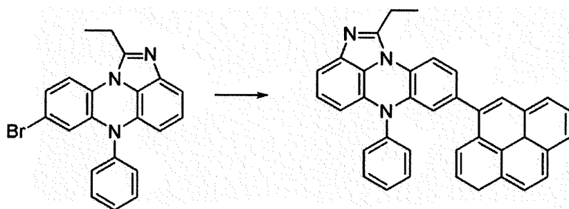
[Compound 2-A]
