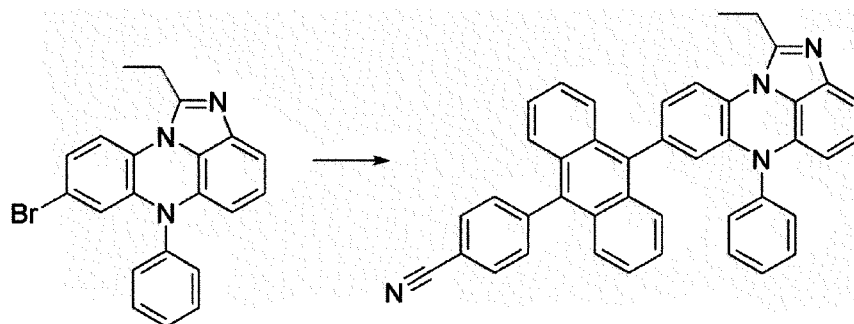
[Compound 2-A]
