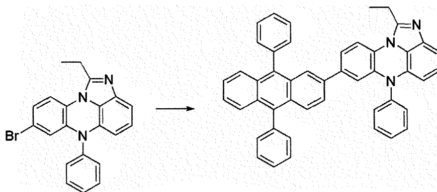
[Compound 2-A]
