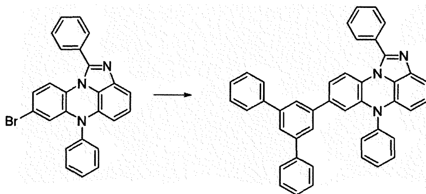
[Compound 14-A]
