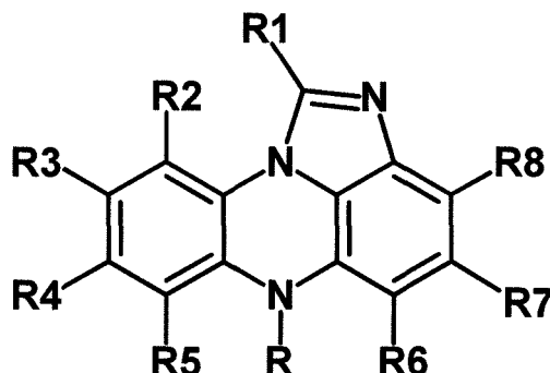
[Chemical Formula 1]
