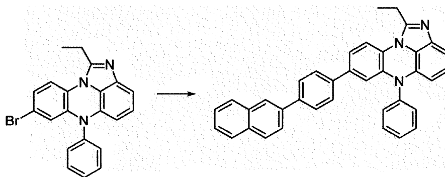
[Compound 2-A]
