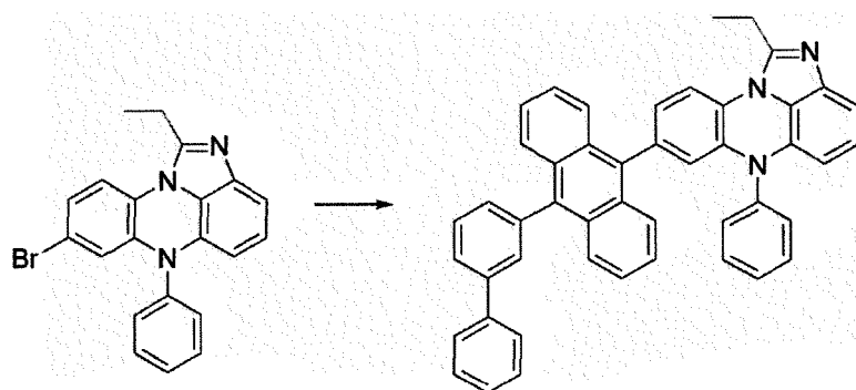
[Compound 2-A]
