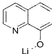
[LiQ]
