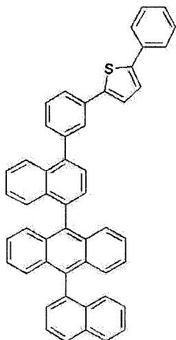
[BH]
