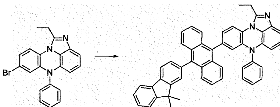
[Compound 2-A]
