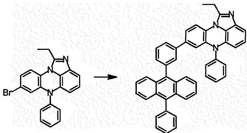
[Compound 2-A]
