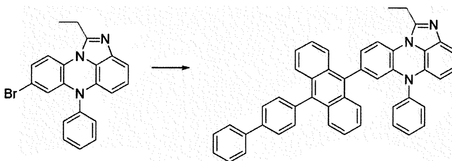
[Compound 2-A]
