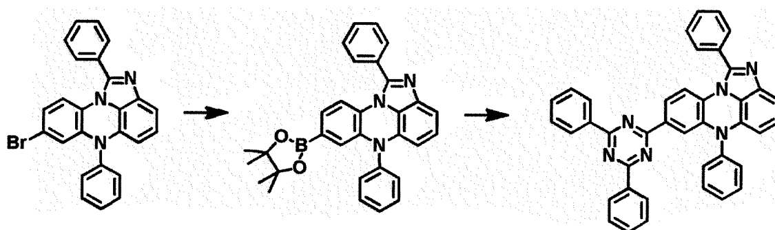
[Compound 14-A]
