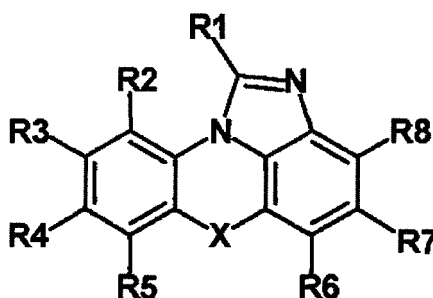
[Chemical Formula 1]
