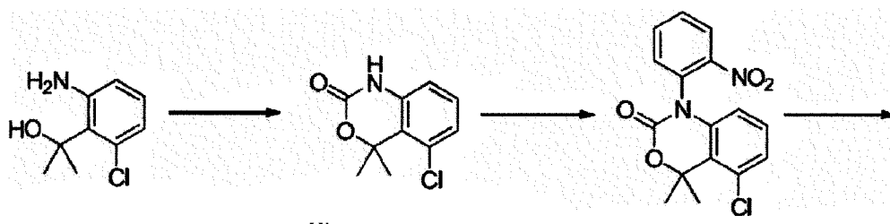
[Compound 9-A]
