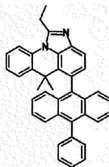
[Chemical Formulae 1-15]
