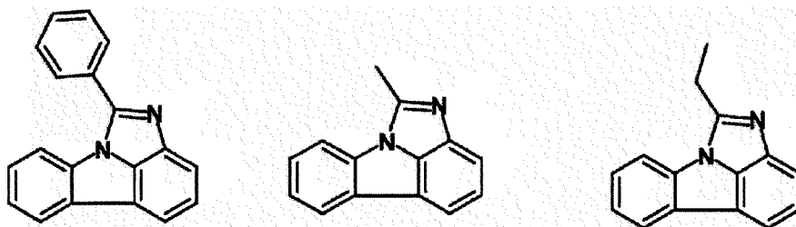
[Chemical Formulae 2-1]
