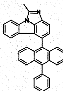
[Chemical Formulae 2-17]
