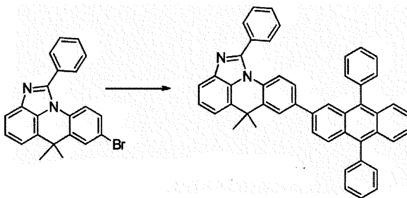
[Compound 3-C]
