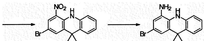
[Compound 1-B]
