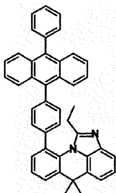
[Chemical Formulae 1-22]
