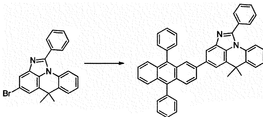
[Compound 6-E]
