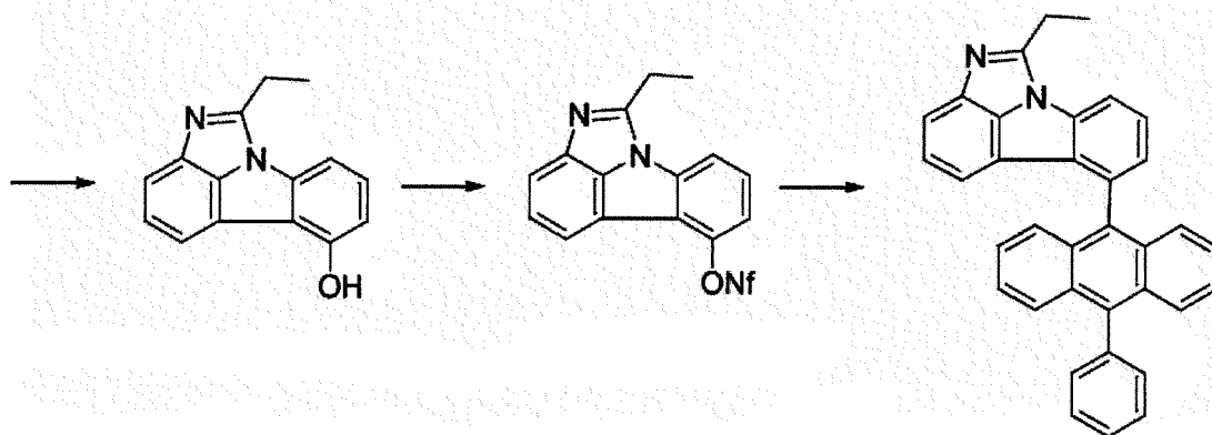
[Compound 18-D]
