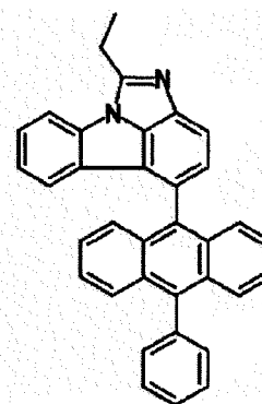
[Chemical Formulae 2-15]
