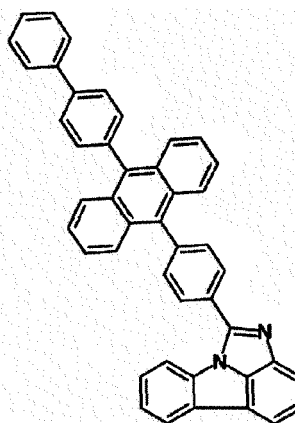
[Chemical Formulae 2-5]
