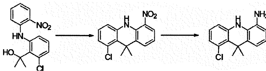
[Compound 9-D]
