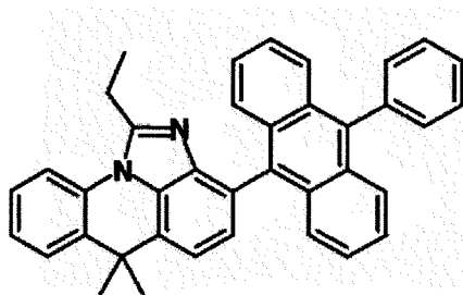
[Chemical Formulae 1-20]
