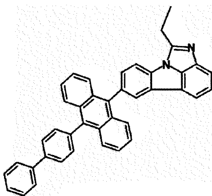
[Chemical Formulae 2-6]
