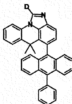
[Chemical Formulae 1-23]
