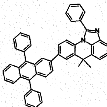
[Chemical Formulae 1-11]
