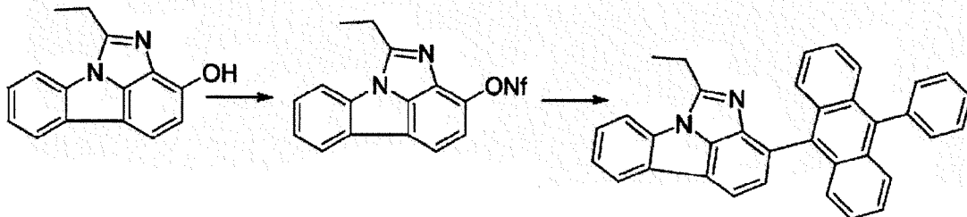
[Compound 19-D]
