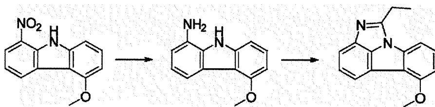
[Compound 18-A]
