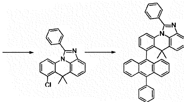
[Compound 9-G]
