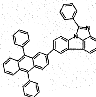
[Chemical Formulae 2-11]
