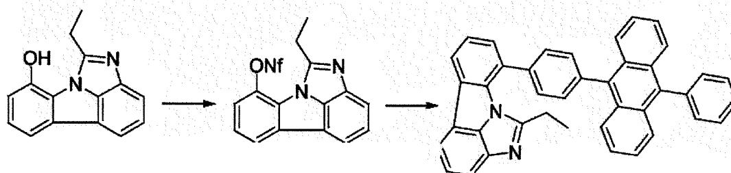
[Compound 21-D]
