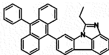
[Chemical Formulae 2-21]
