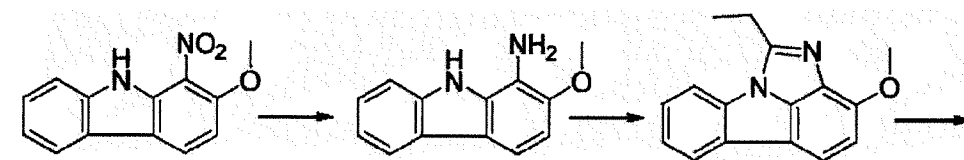
[Compound 19-A]
