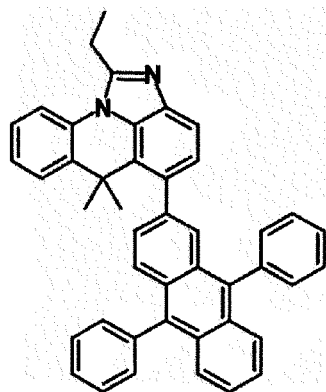
[Chemical Formulae 1-16]
