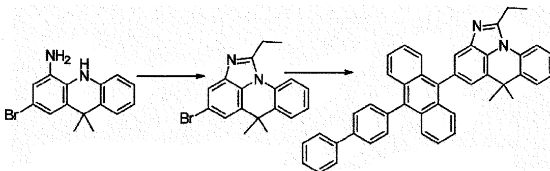
[Compound 6-D]
