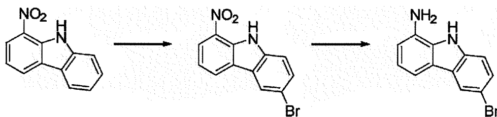
[Compound 13-A]
