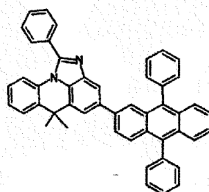
[Chemical Formulae 1-9]
