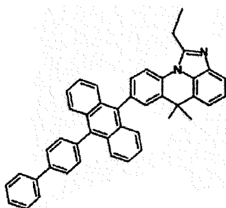
[Chemical Formulae 1-8]
