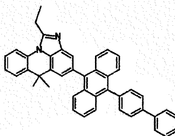
[Chemical Formulae 1-7]
