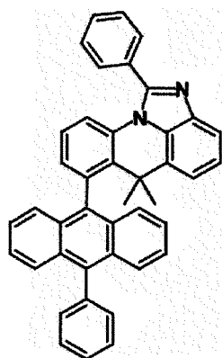
[Chemical Formulae 1-18]
