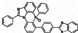
[Chemical Formula 2-6-46] [Chemical Formula 2-6-47] [Chemical Formula 2-6-48]
