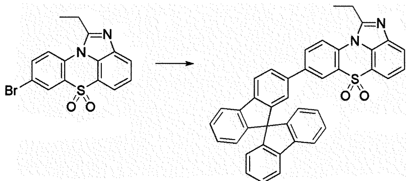
[Compound 2-B]
