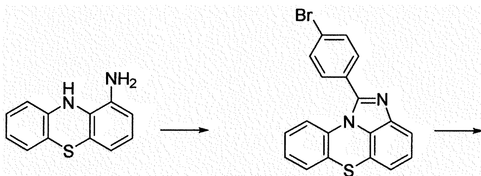
[Compound 15-A]
