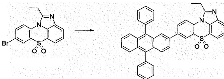
[Compound 2-B]
