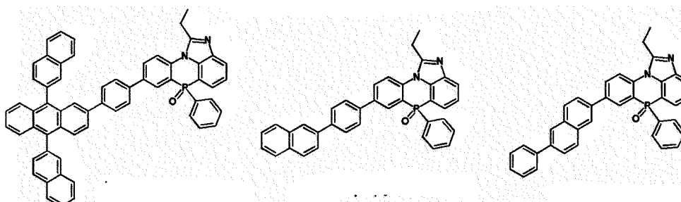
[Chemical Formula 2-3-25] [Chemical Formula 2-3-26] [Chemical Formula 2-3-27]
