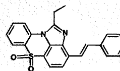
[Chemical Formula 1-11-16] [Chemical Formula 1-11-17] [Chemical Formula 1-11-18]
