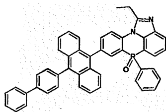
[Chemical Formula 2-3-4] [Chemical Formula 2-3-5] [Chemical Formula 2-3-6]
