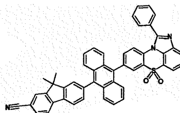
[Chemical Formula 1-4-13] [Chemical Formula 1-4-14] [Chemical Formula 1-4-15]
