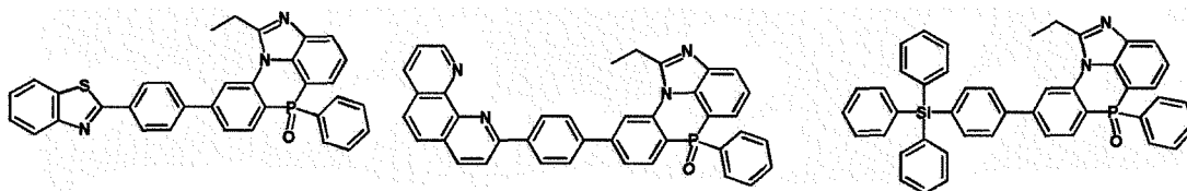
[Chemical Formula 2-7-46] [Chemical Formula 2-7-47] [Chemical Formula 2-7-48]
