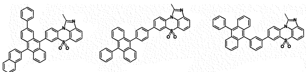
[Chemical Formula 1-2-16] [Chemical Formula 1-2-17] [Chemical Formula 1-2-18]
