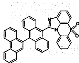
[Chemical Formula 1-5-7] [Chemical Formula 1-5-8] [Chemical Formula 1-5-9]
