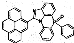
[Chemical Formula 2-5-28] [Chemical Formula 2-5-29] [Chemical Formula 2-5-30]
