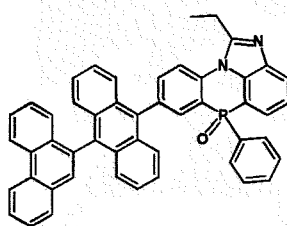
[Chemical Formula 2-3-7] [Chemical Formula 2-3-8] [Chemical Formula 2-3-9]
