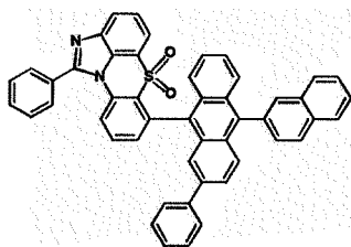
[Chemical Formula 1-6-16] [Chemical Formula 1-6-17] [Chemical Formula 1-6-18]
