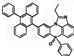
[Chemical Formula 2-7-1] [Chemical Formula 2-7-2] [Chemical Formula 2-7-3]
