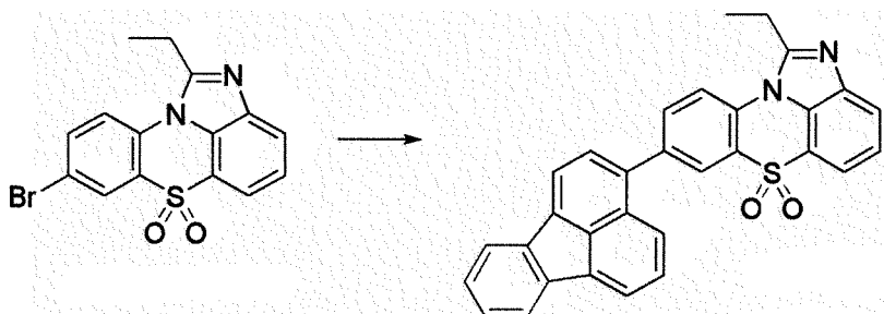
[Compound 2-B]
