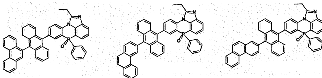
[Chemical Formula 2-3-7] [Chemical Formula 2-3-8] [Chemical Formula 2-3-9]
