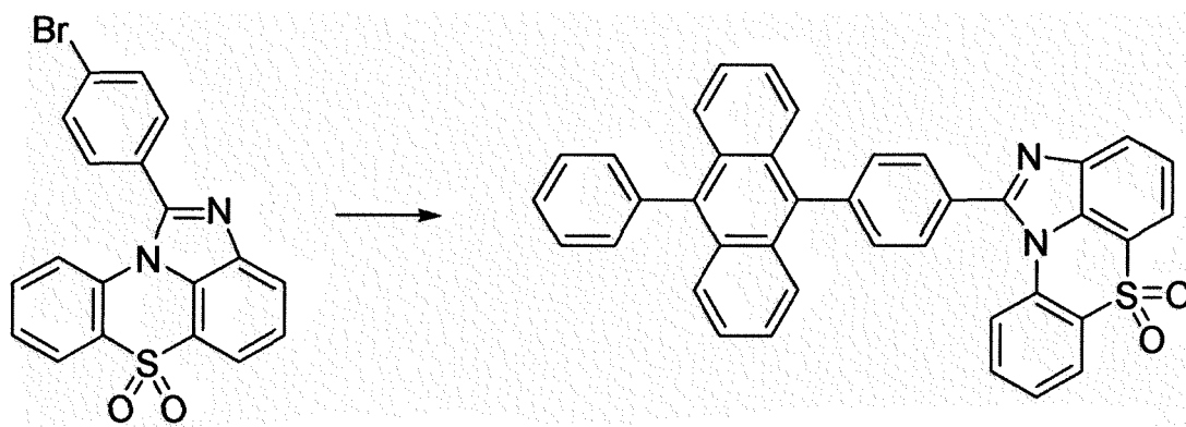
[Compound 15-C]
