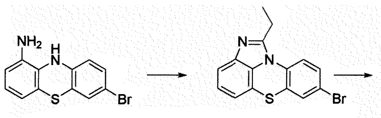
[Compound 1-C]
