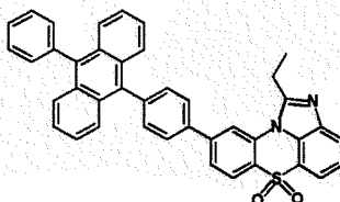
[Chemical Formula 1-7-16] [Chemical Formula 1-7-17] [Chemical Formula 1-7-18]
