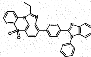
[Chemical Formula 1-11-7] [Chemical Formula 1-11-8] [Chemical Formula 1-11-9]
