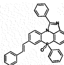
[Chemical Formula 2-4-52] [Chemical Formula 2-4-53] [Chemical Formula 2-4-54]
