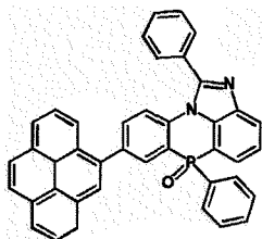
[Chemical Formula 2-4-28]
