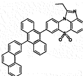
[Chemical Formula 1-3-7] [Chemical Formula 1-3-8] [Chemical Formula 1-3-9]
