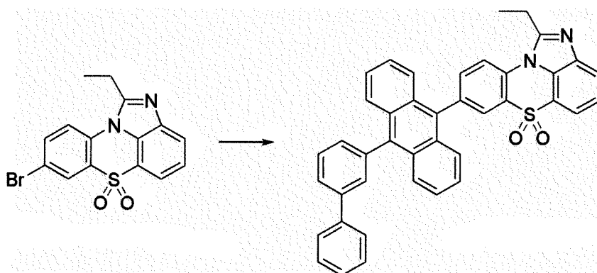
[Compound 2-B]
