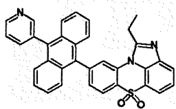
[Chemical Formula 1-7-10] [Chemical Formula 1-7-11] [Chemical Formula 1-7-12]
