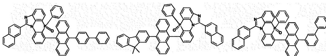
[Chemical Formula 2-6-4] [Chemical Formula 2-6-5] [Chemical Formula 2-6-6]
