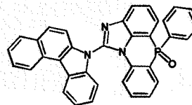
[Chemical Formula 2-5-49] [Chemical Formula 2-5-50] [Chemical Formula 2-5-51]
