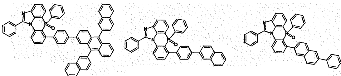
[Chemical Formula 2-6-25] [Chemical Formula 2-6-26] [Chemical Formula 2-6-27]
