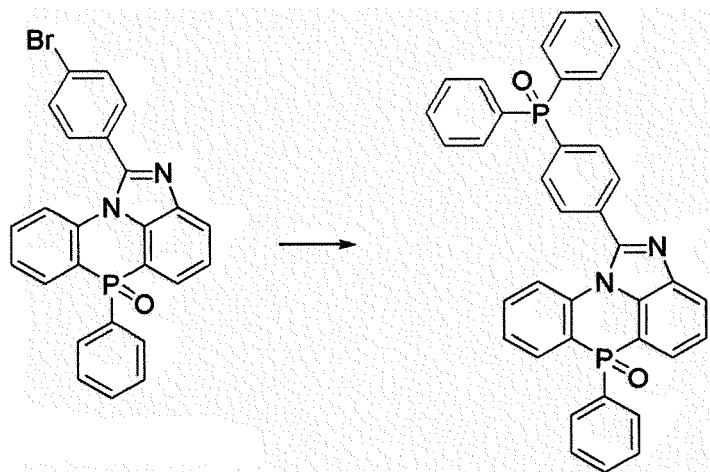
[Compound 2-1-G]
