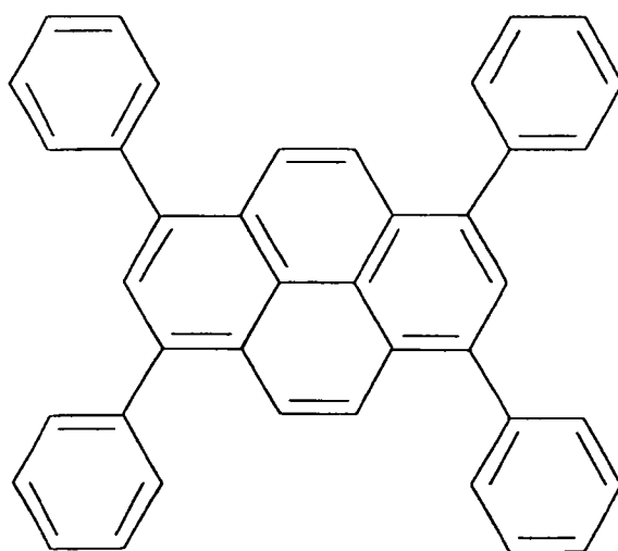
1,3,6,8-tetraphenylpyrene
