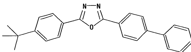
2-(4-tert-butylphenyl)-5-(4-biphenyl)-1,3,4-oxadiazole
