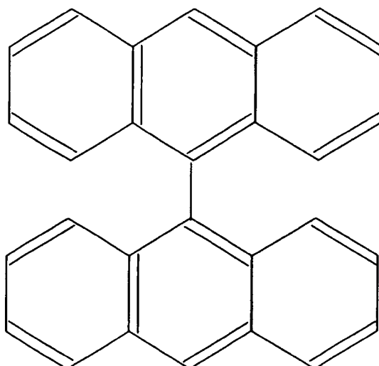
9,9'-bianthryl
