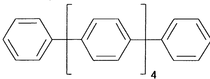
p-sexiphenyl
