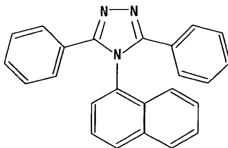
3-phenyl-4-(1-naphthyl)-5-phenyl-1,2,4-triazole
