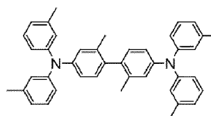
HMTDP
