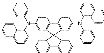
Spiro-NPB
