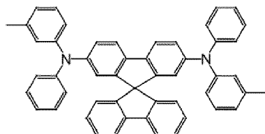
Spiro-TPD
