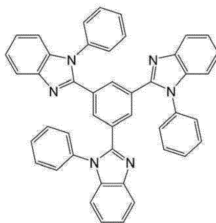
TPBi
