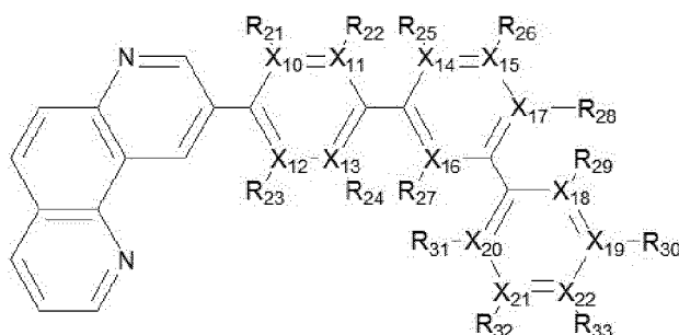
[Chemical Formula 13]
