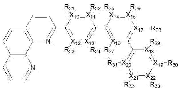
[Chemical Formula 11]
