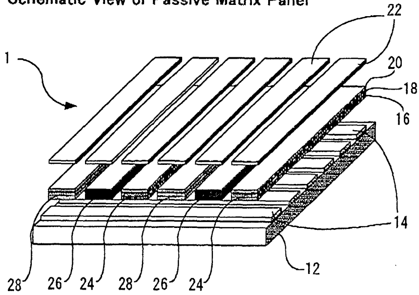
Schematic View of Passive Matrix Panel
