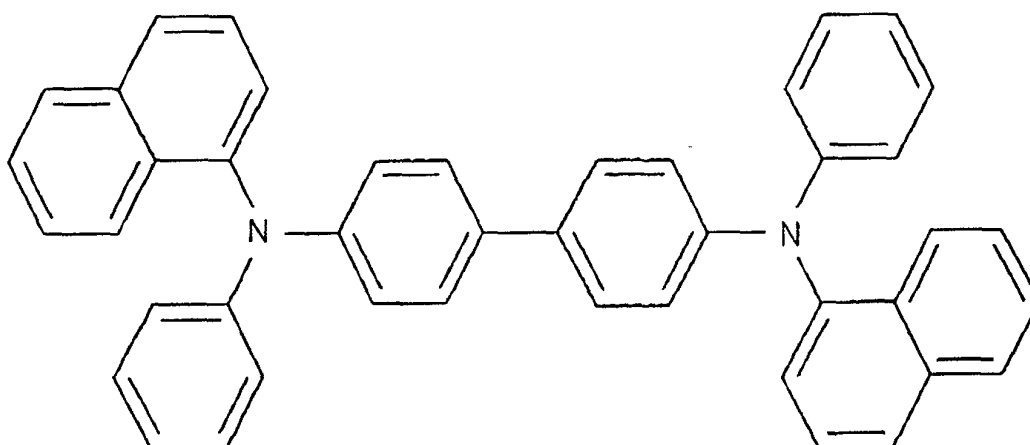
NPD
