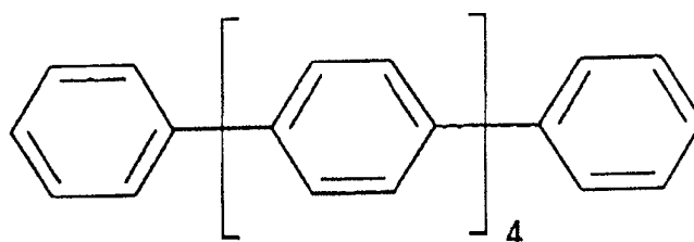
P-sexiphenyl
