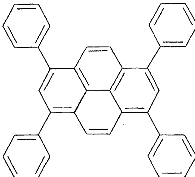
1,3,6,8-tetraphenylpyrene
