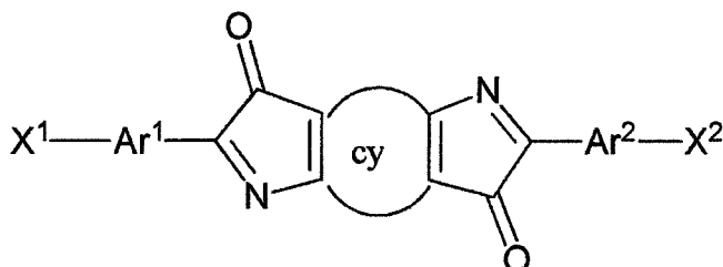
Formula (6)
