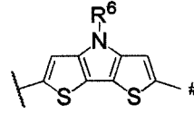
Formula (5-3)
