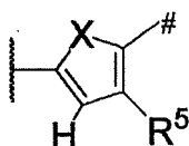
Formula (4-1A)
