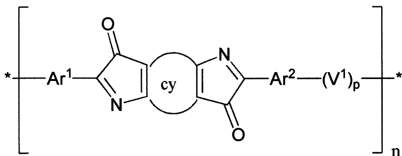
Formula (1-2B)
