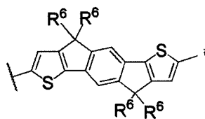
Formula (5-7)
