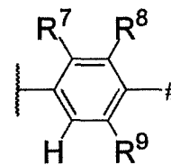
Formula (4-3)
