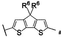
Formula (5-2)
