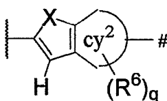
Formula (4-2)
