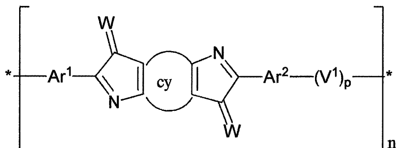
Formula (1-2')
