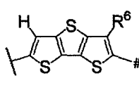
Formula (5-6)
