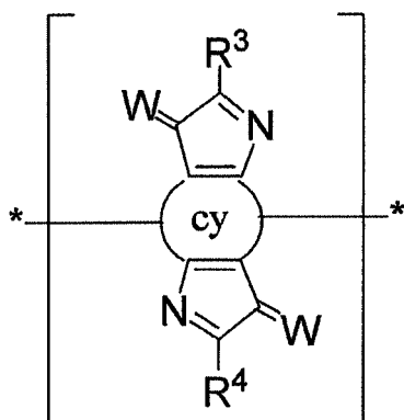
Formula (1-3)
