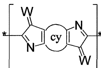
Formula (1-2)
