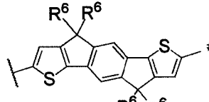
Formula (5-7)
