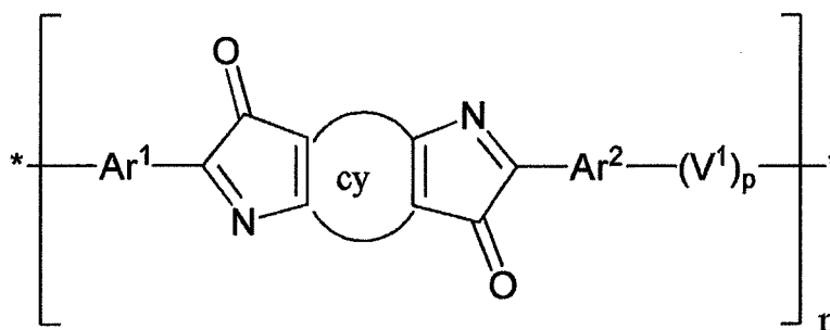
Formula (1-2B)
