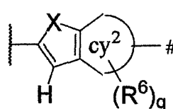
Formula (4-2)
