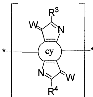
Formula (1-3)
