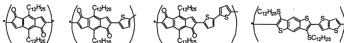
Comparative compound 1
