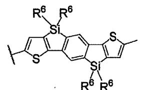
Formula (5-8)
