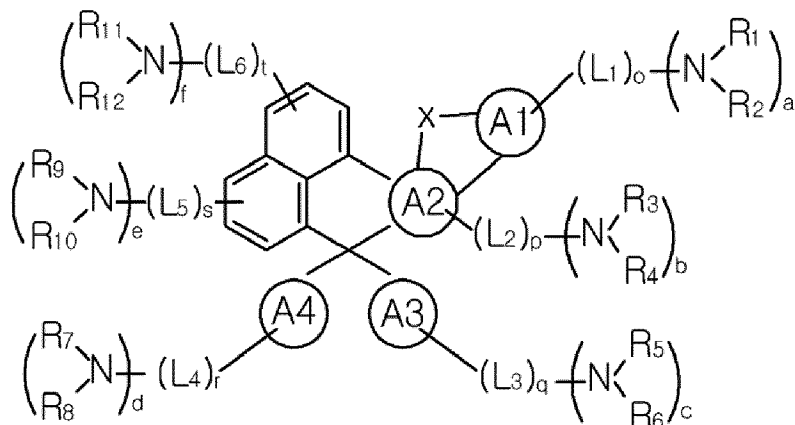
Chemical Formula 1
