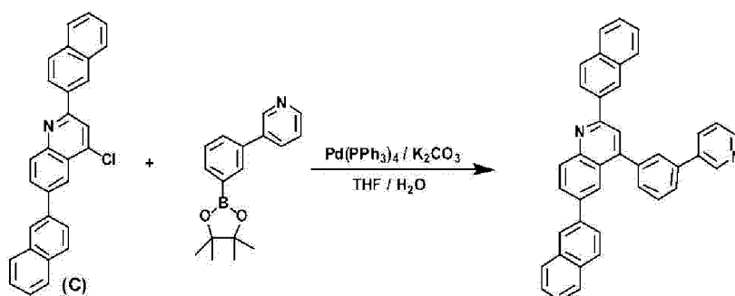
[Reaction Scheme 8]
