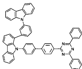
[Chemical Formula 43]
