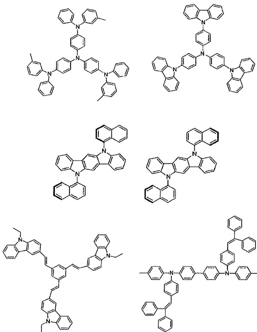
[Chemical Formula 59]
