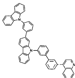
[Chemical Formula 29]
