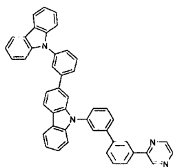
[Chemical Formula 28]
