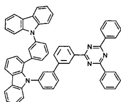
[Chemical Formula 45]
