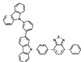
[Chemical Formula 36]
