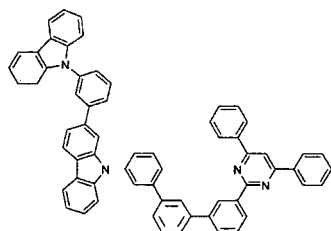
[Chemical Formula 35]
