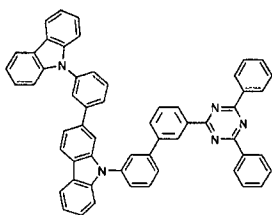
[Chemical Formula 14]
