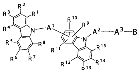
[Chemical Formula 1]
